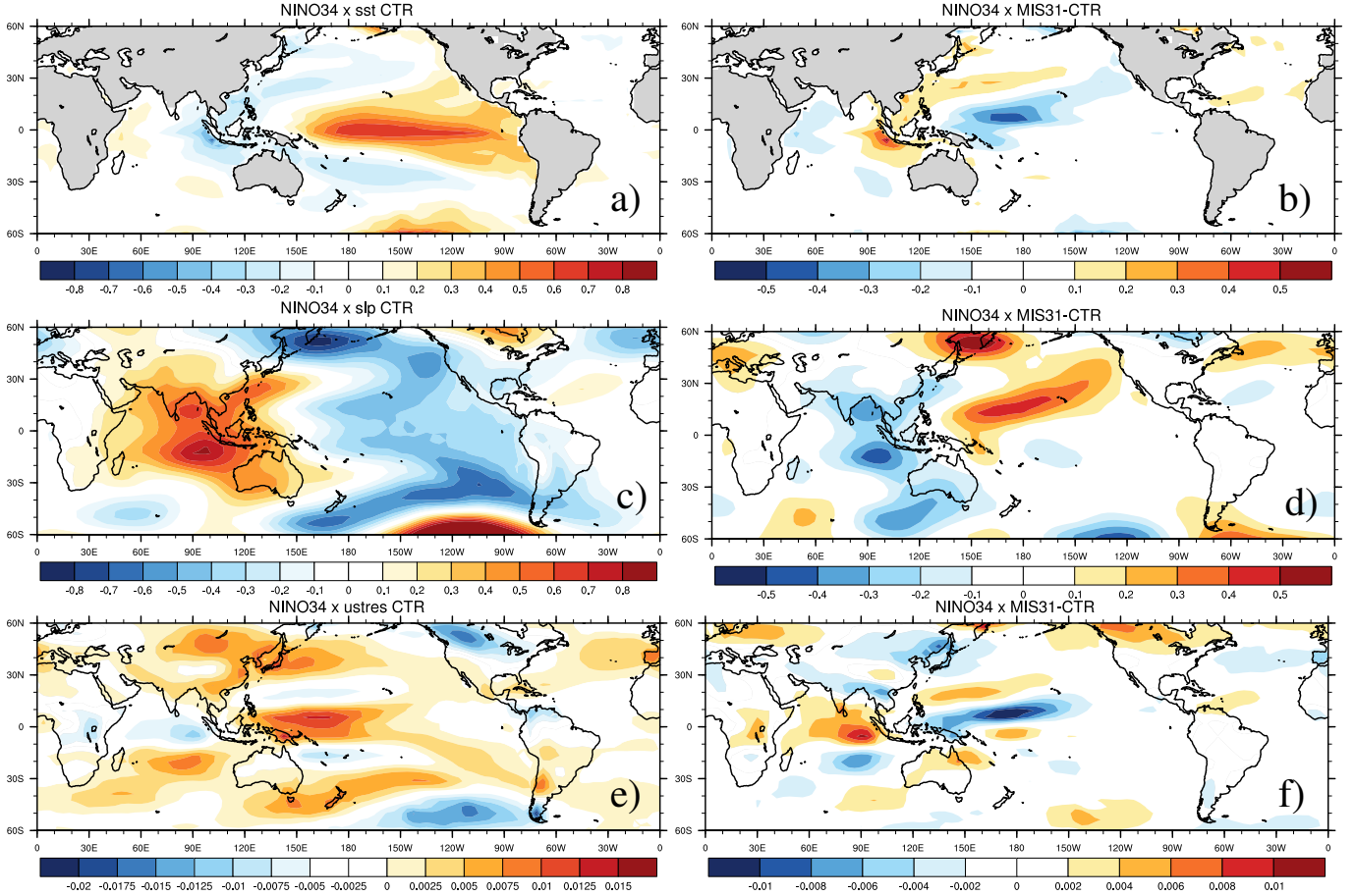
Figure 4. (a) is the leading EOF of SST anomalies for the CTR simulation displayed as amplitudes ( ^{\circ}\text{C} ) by regressing hemispheric SST anomalies upon the Niño34 timeseries. (b) shows SST differences between the MIS31 and CTR regressed patterns. (c) and (d) are as in (a) and (b) but for SLP (mb). (e) and (f) as in (a) and (b) but for zonal wind stress ( \text{Nm}^{-2} ). Please note that Figures are shown with distinct labels
