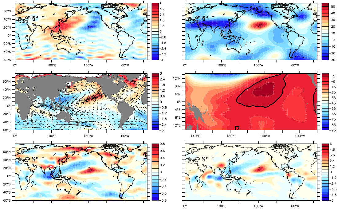
Figure 1. a) Annual differences between MIS31 and CTR runs for \text{SLP}_e and b) for Z200 (mb). c) shows differences of monthly SST ( ^{\circ}\text{C} ) and windstress (vector, \text{Nm}^{-2} ) between MIS31 and CTR runs. d) differences of thermocline depth between MIS31 and CTR simulation (meter). e) and f) show differences between MIS31 and CTR zonal windstress ( \text{Nm}^{-2} ), and precipitation differences between MIS31 and CTR runs (mm/day). g) is the Sverdrup transport in the CTR and h) the difference between the Sverdrup transport in the MIS31 and CTR runs.
