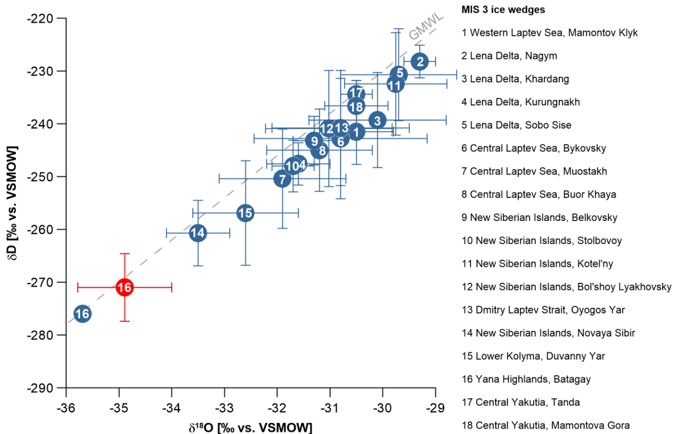
5 Figure 7. Comparison of stable isotope data from Siberian ice wedges attributed to the MIS 3 interstadial (about 50 to 30 kyr), comprising data from the western Laptev Sea (Magens, 2005), the Lena River Delta (Schirrmeister et al., 2003; Schirrmeister et al., 2011a; Wetterich et al., 2008; Opel, unpublished), the central Laptev Sea (Meyer et al., 2002a; Meyer/Opel, unpublished; Schirrmeister et al., 2017), the New Siberian Islands and the Dmitry Laptev Strait (Schirrmeister, unpublished; Wetterich et al., 2014; Opel et al., 2017b), the Kolyma Lowland (Strauss, 2010), the Yana Highlands (this study; Vasil'chuk et al., 2017), and central Yakutia (Schirrmeister, unpublished; Popp et al., 2006). The new data from Batagay are marked in red. Further information is given in Table S3.
