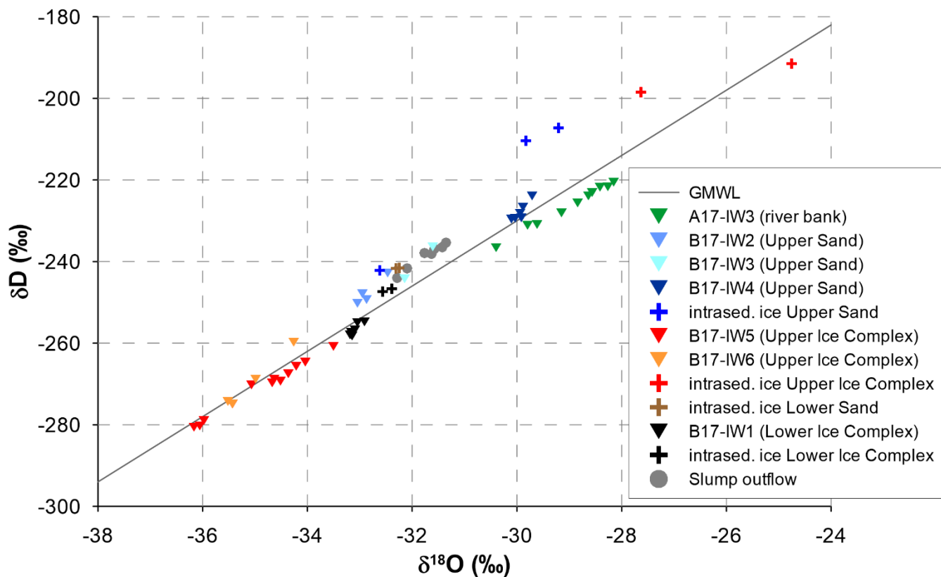
5 Figure 6. Co-isotopic \delta^{18}\text{O} – \delta\text{D} diagram of ice wedges and intrasedimental ice sampled at the Batagay megaslump and the Adycha River. The data from the Batagay megaslump outflow samples record an integrated signal of the entire Batagay permafrost sequence and modern precipitation.
