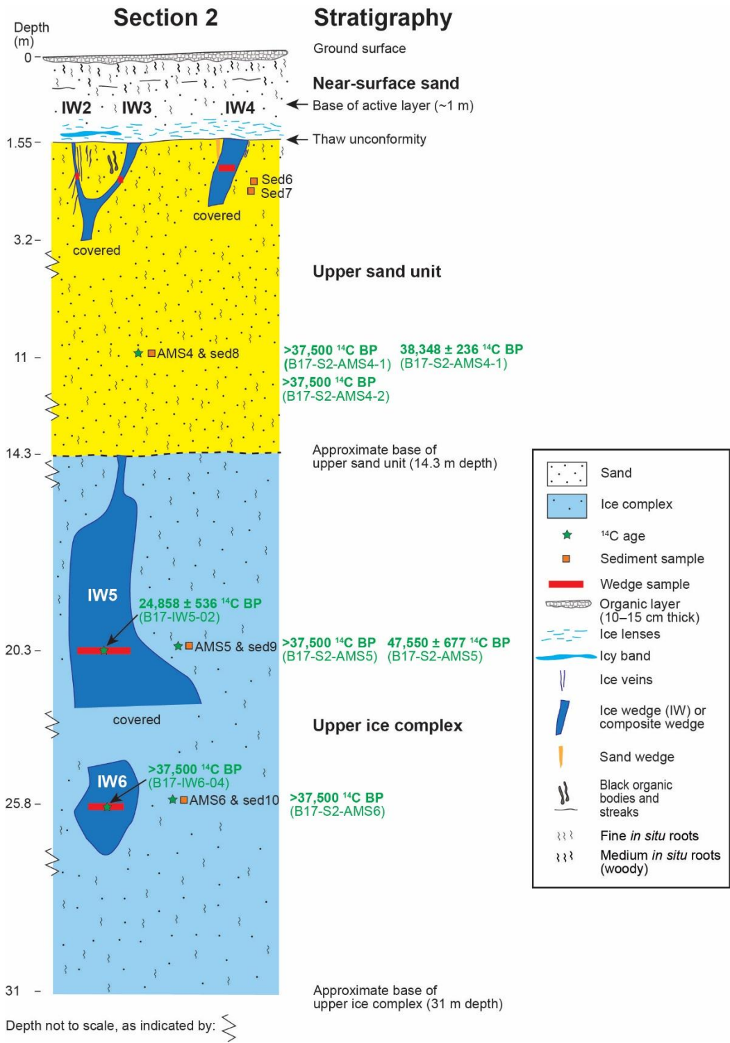
Figure 5. Schematic cryostratigraphic sketch of Section 2, Batagay megalump.
