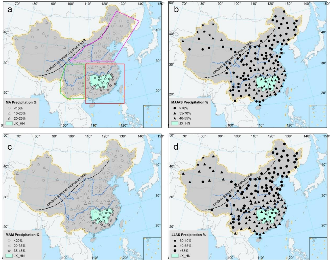
190 Figure 2. The percentage of spring (a, March to April) and EASM (b, May to September) precipitation amount relative to the annual precipitation amount in China. Figures c and d are similar to a and b, except that spring precipitation is shown from March to May in c and EASM precipitation between June and 195 Ji'an, Ganzhou, Changsha, Yueyang, Hengyang, Chenzhou, Xinning) in the Jiangxi Province and the eastern Hunan Province were used to examine the relationship between ocean-atmospheric circulation, precipitation amount and \delta^{18}\text{O} in the SPR region. The red, pink and green polygons in panel a indicate southeastern, northern and southwestern regions of the MRC, respectively.
