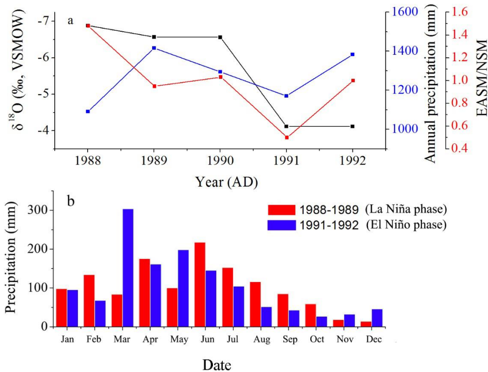
360 Figure 5. Comparison between ENSO events, precipitation amount and \delta^{18}\text{O}_w at the Changsha GNIP station for the period 1988-1992. (a) Comparison between annual precipitation amount, \delta^{18}\text{O}_w , and the EASM/NSM ratio. (b) Comparison of mean monthly precipitation amount between La Niña (1988-1989) and El Niño (1991-1992) years. In this calculation, the temporal coverage of the annual precipitation and the precipitation \delta^{18}\text{O}_w is from January to December, the EASM precipitation is from May to September 365 and the NSM precipitation is from January to April and from October to December.
