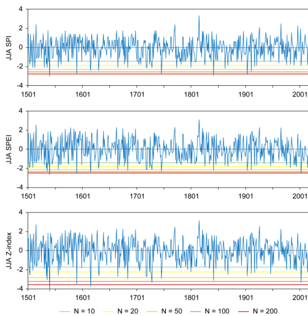
Figure 2. Fluctuations in JJA SPI, JJA SPEI and JJA Z-index in the Czech Lands in the 1501–2017 period. Coloured horizontal lines mark the limits for estimation of extreme droughts with return periods of N = 10, 20, 50, 100, and 200 years.
