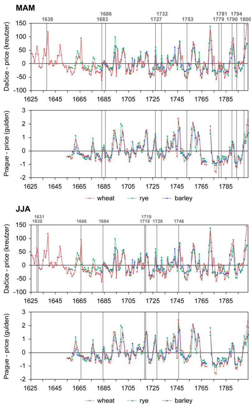
5 Figure 8. Deviations in grain prices (wheat, rye and barley) in Dačice for 1625–1803 (Brázdil and Durdáková, 2000) and in Prague in 1655–1803 (Schebek, 1873) with identification of extremely dry MAM and JJA seasons.
