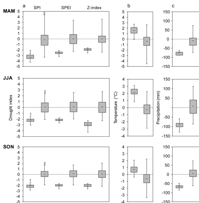
Figure 3. Box-plots (maximum and minimum, upper and lower quartile, mean) of Czech drought indices (a), central European temperatures (b) and Czech precipitation (c) in MAM, JJA and SON: 1 – 5 dry years with N \geq 20 years, 2 – remaining years 1501–1803. Temperatures and precipitation are expressed as anomalies with respect to the 1961–1990 reference period.
