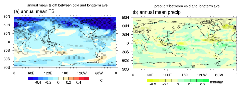
Figure A Spatial distribution of the annual mean (a) surface temperature and (b) precipitation anomalies of the cold periods against the long-term average of 5000-3000 BP derived from the TraCE-ALL run. Those regions where significant above 95% confidence level are dotted.
