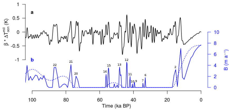
Figure 4. Evolution of a) millennial-scale subsurface oceanic temperature as defined in Eq. 6 to force the TOT max simulation and b) the resulting submarine melting used in both TOT max (solid line) and ORB max (dashed line) simulations for the last 100 ka. Submarine melt peaks are associated with their corresponding Greenland Stadials (GS).
