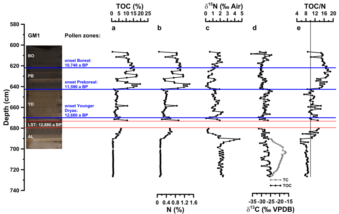
Fig. 3: (a) Depth profiles of total organic carbon (TOC), (b) total nitrogen (N), (c) bulk stable nitrogen isotope composition ( \delta^{15}\text{N} ), (d) stable carbon isotope composition of total carbon (TC) and TOC ( \delta^{13}\text{C}_{\text{TC}} , \delta^{13}\text{C}_{\text{TOC}} ) and (e) carbon to nitrogen atomic ratio (TOC/N). The vertical line in (e) indicates a TOC/N atomic ratio threshold of 10 (Meyers, 2003). AL = Allerød, YD = Younger Dryas, PB = Preboreal and BO = Boreal.
