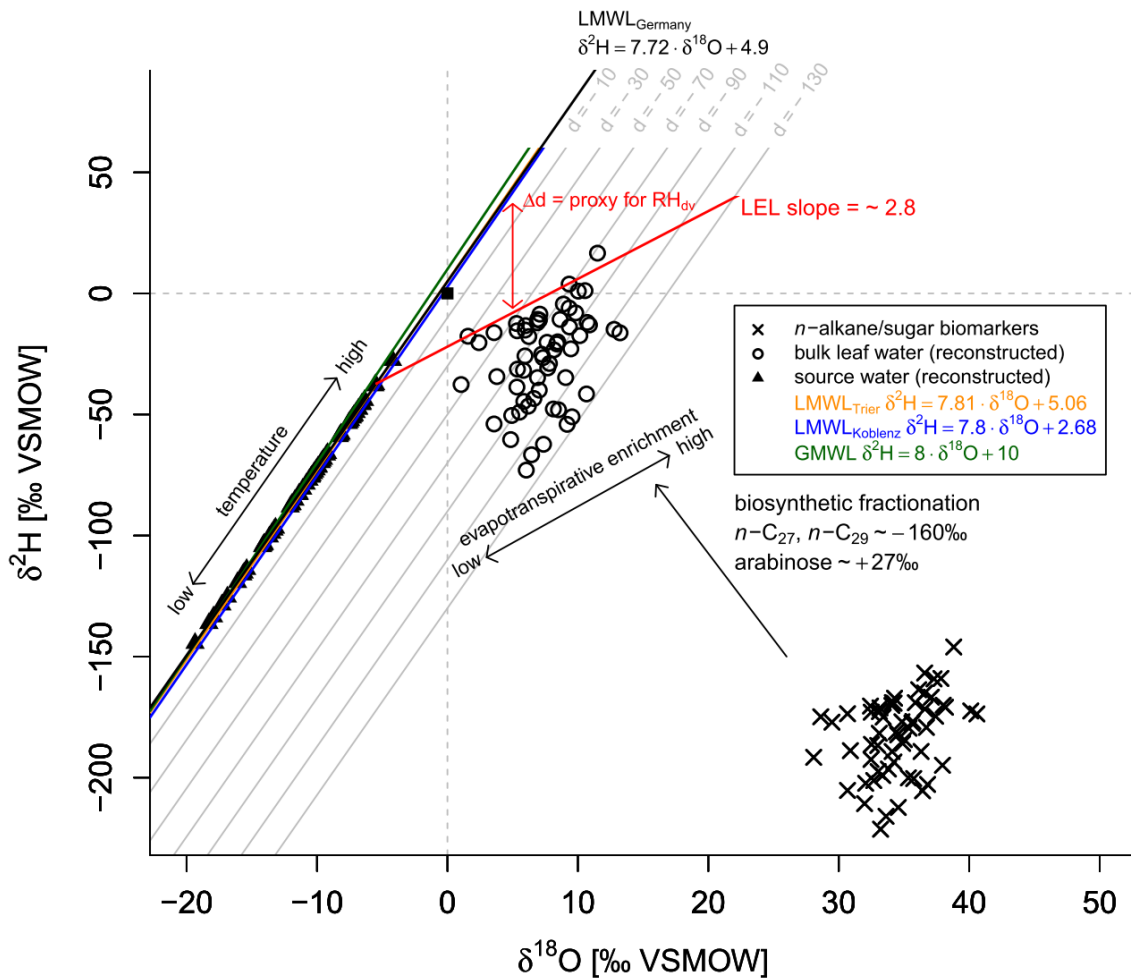
Fig. 5: Conceptual framework of the coupled \delta^2\text{H}_{n\text{-alkane}}\text{-}\delta^{18}\text{O}_{\text{sugar}} paleohygrometer approach displayed as \delta^{18}\text{O}\text{-}\delta^2\text{H} diagram showing the measured n -alkanes (weighted mean of n\text{-C}_{27} and n\text{-C}_{29} ) and sugar (arabinose) biomarkers (black crosses), the reconstructed leaf water (open circles), the global meteoric water line (GMWL, green line) and the local meteoric water lines of Germany (LMWL Germany , black line), Trier (LMWL Trier , yellow line) and Koblenz (LMWL Koblenz , blue line). The black arrows indicate natural processes of evapotranspirative enrichment of leaf water along local evaporation lines (LEL), biosynthetic fractionation during biomarker synthesis and the temperature effect on the source water isotope composition (~precipitation). Grey lines indicate the parallel distance between the individual reconstructed evaporative site leaf water points and the LMWL Germany , expressed as d = \delta^2\text{H} - 7.72 \cdot \delta^{18}\text{O} . The difference between the d -excesses of the leaf water and source water can serve as proxy for mean daytime vegetation period relative humidity ( \text{RH}_{\text{dv}} ; red double arrow).
