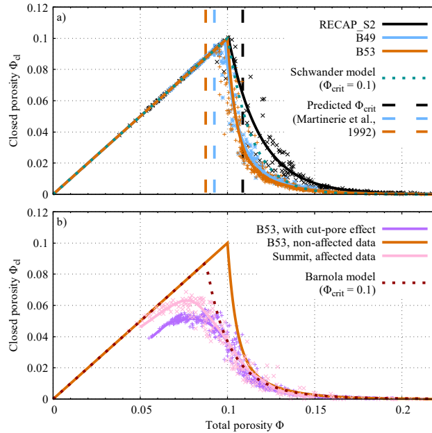
Figure 2. Closed versus total porosity for a) the analyzed cores in comparison with commonly expected values and b) B53 ignoring cut pores compared to previous results from Summit, Greenland (Schwander et al., 1993). The solid lines indicate least squares fits for the respective core, the short-dashed lines represent model results (Schwander, 1989; Goujon et al., 2003) for the given parameters and the long-dashed lines mark the critical porosity values predicted by the previously observed temperature dependence (Martinerie et al., 1992).
