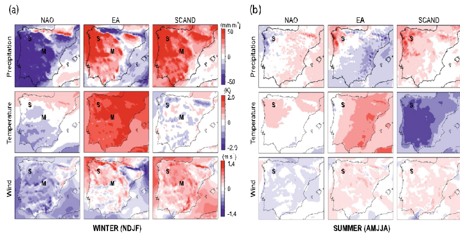
Figure 1 (Figure 5 of Hernández et al., (2015)). NAO, EA and SCAND modes effect on the mean pre- wind speed. 1 month lag time winter months (NDJF avg), and summer months (AMJJA avg).
