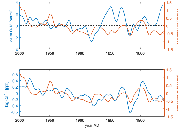
Figure 6. Comparison of KCC \delta^{18}\text{O} and \text{Ca}^{2+} against the CG modified instrumental temperature (orange), shown in top and bottom, respectively, and covering the full instrumental period back to 1760 AD. Shown are anomalies relative to the respective 2000-1860 AD mean, and as decadal trends obtained from Gaussian smoothing.
