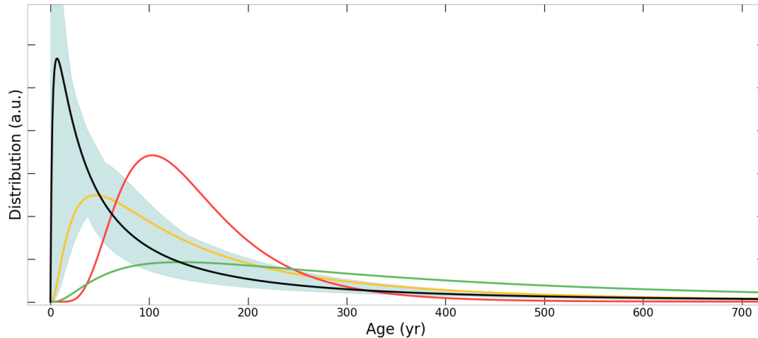
Figure 6. Gas Age Distributions. In black: the Vostok GAD during the DO-17 estimated with our optimization scheme, the uncertainty envelope is shown in light blue. In yellow: a log-normal fit to the modern conditions Vostok GAD from Witrant et al. (2012). In red: the estimated Dome C GAD during B/A from Köhler et al. (2015). In green: the estimated Dome C GAD during LGM from Köhler et al. (2011).
