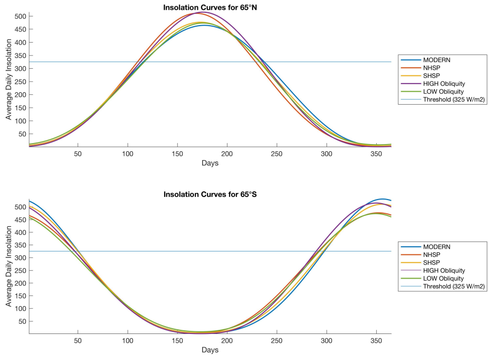
Figure 3: Insolation curves for different orbits for Northern and Southern Hemispheres. The horizontal line shows the threshold of 325 W/m 2 used to define summer. And day with average insolation higher than 325 W/m 2 is considered as summer. Defining summer this way accounts for the variation in duration and timing of summer at different orbits.
