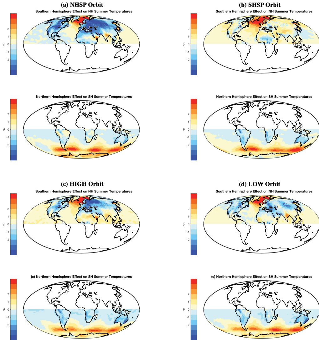
Figure 4: Hemispheric Effects on Summer Temperature (summer defined by an insolation threshold) for different orbits
