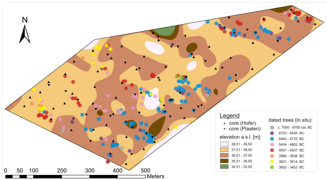
5 Figure 6: Elevations a.s.l. of the mineral base (sand) below the peat. Regularized spline interpolation of 99 measurements. The elevations are interpolated using a regularized spline. The actual measurements range from 36,42 to 38,16 m a.s.l.; thereby, the first and the last elevation class (green, below 35,50 m a.s.l., and white, above 38,51 m a.s.l.) are products of extrapolation only. The coring points are indicated by triangles. The dated in situ trees are shown as circles, for each chronology segment (Table 1) in a different colour (C14: grey, A1: dark violet, A2: blue, B: pink, C: red, D: orange, E: yellow, F: green).
