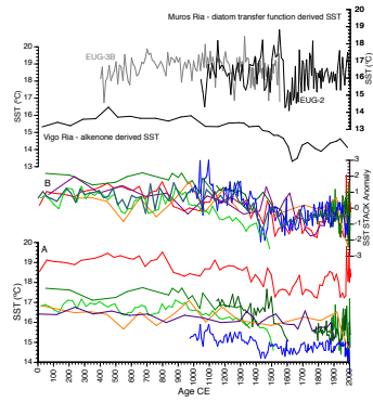
Figure 3R1 - Comparison of the SST records of the various cores (A) used for the Iberian Margin STACK construction (B), with the Ria de Vigo Ria alkanone-derived SST and the Ria de Muros diatom-derived SST for sites EUG-2 and EUG-3B (Straykowski, 2009).
