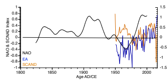
Figure 2R1 - Instrumentally derived NAO, EA and SCAND index.
