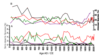
Figure 4R1 - Variability of the semi-desertic plants percent abundance (A); arboreal species percent abundance (B) along cores Minho, Tejo, Algarve and Vigo (black line);
