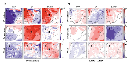
Fig 5 of Hernandez et al., (2015) NAO, EA and SCAND modes on the mean precipitation, temperature and wind speed. 1 month lag time winter months (NDJF avg), and summer months (AMJJJA avg).
