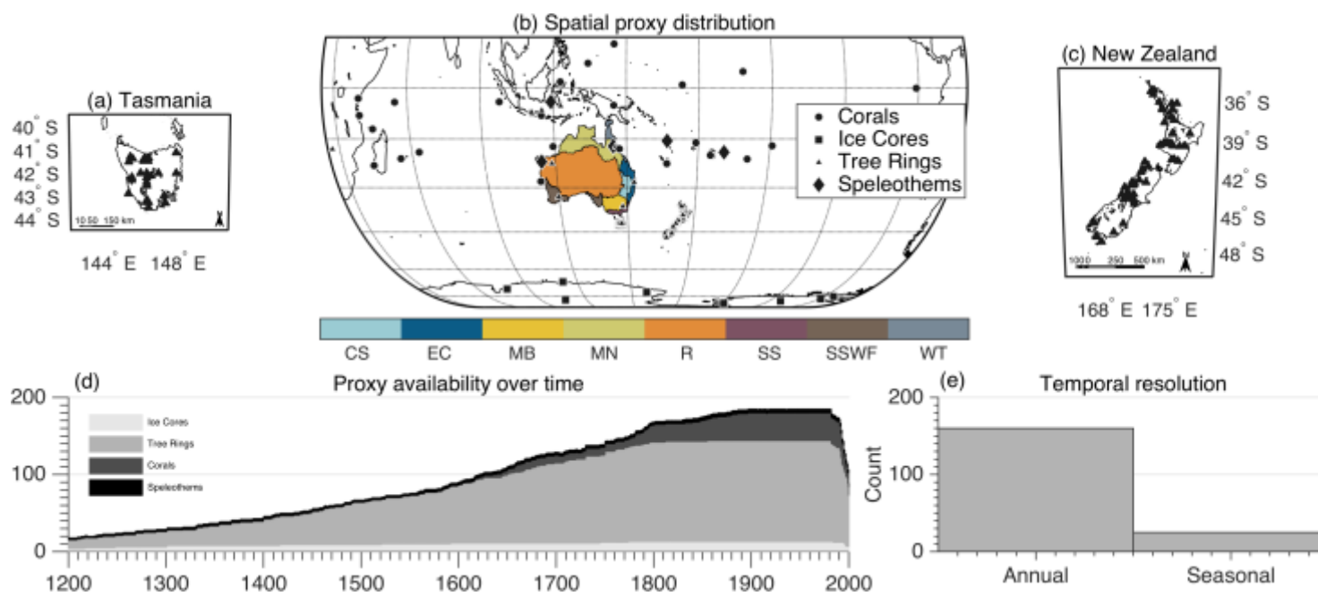
Figure 1. Overview of Southern Hemisphere multi-proxy network. a) Spatial distribution of tree-ring sites in Tasmania b) Spatial distribution of 202 individual proxy records by archive type; National Resource Management (NRM) clusters shown on Australian continent corresponding to abbreviations 5 given in Table 1 a. c) Spatial distribution of tree-ring sites in New Zealand d) Record availability as a function of archive and time period covered, e) Temporal resolution of the palaeoclimate records
