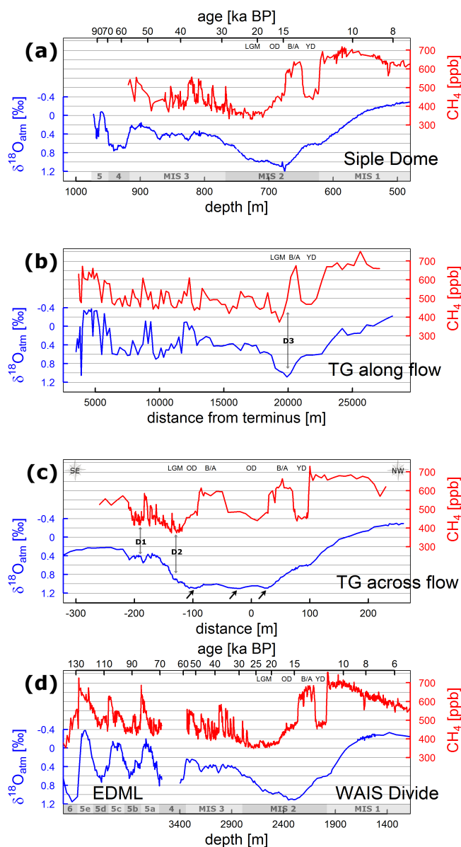
Figure 3. \delta^{18}\text{O}_{\text{atm}} (blue, note reversed scale) and methane (red) records from deep ice cores (Siple Dome (Brook et al., 2005; Severinghaus et al., 2009), WD (Buizert et al., 2015), EDML (Capron et al., 2010; Schilt et al., 2010)) and from Taylor Glacier (across-flow, along-flow). TG along-flow methane data is based on lab analyses only, whereas the across-flow data is a combination of lab and field analyses. For TG across-flow, the 0 m point is arbitrarily chosen at a conspicuous circular feature (Fig. 5a), and the threefold \delta^{18}\text{O}_{\text{atm}} maximum is highlighted with arrows. The approximate locations of the three deep cores D1, D2, and D3 are shown in (b) and (c). The intersection point of the two TG sampling lines is at -240 m on the across-flow scale, and at 13.5 km on the along-flow scale. Distinct climate periods of the deglaciation (top of each panel) and Marine Isotope Stages (MIS, bottom) are indicated.
