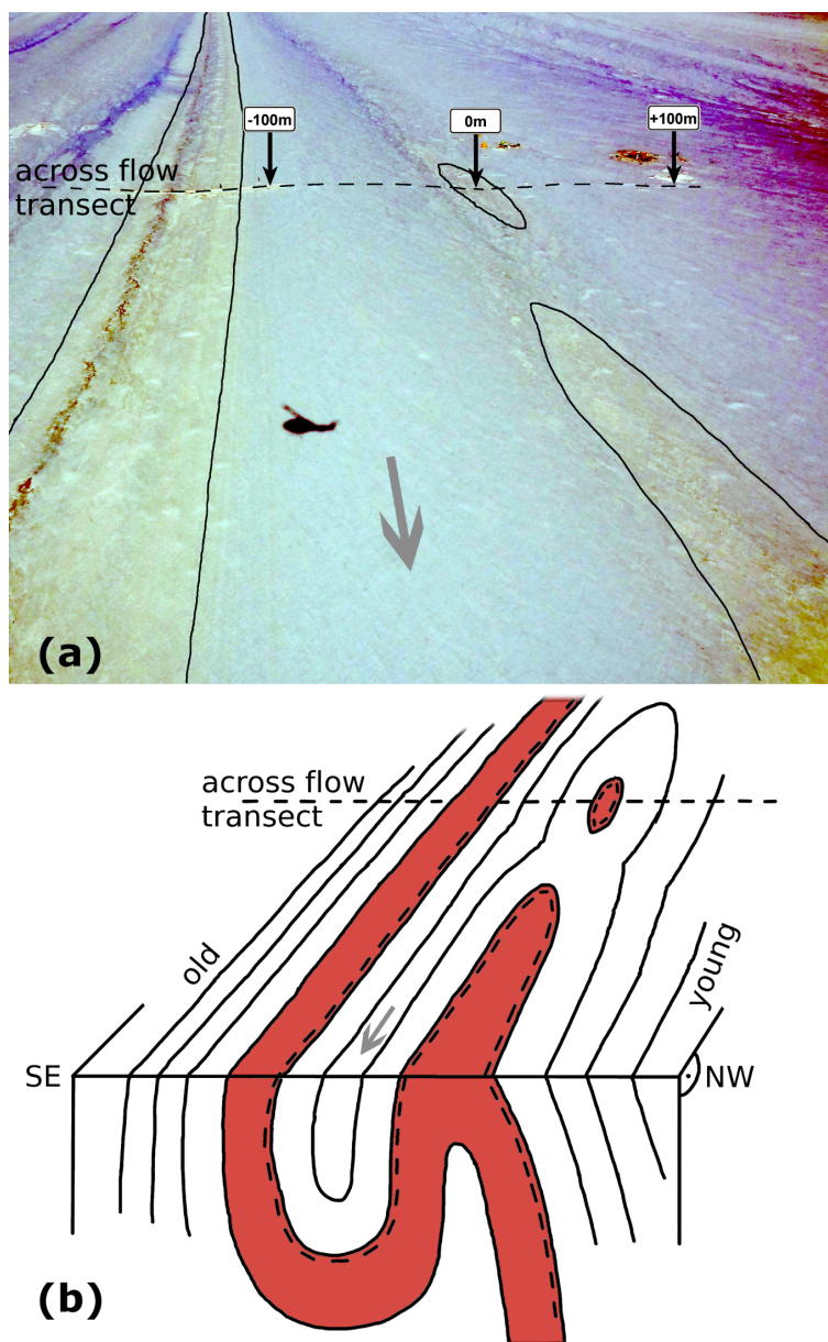
Figure 5. Folding on Taylor Glacier. (a) Photo of the across-flow transect sampling area showing two limbs of the dusty band. Color settings were adjusted to enhance the color differences. The solid black line marks the approximate boundary of the dusty band. The dashed black line marks the across-glacier transect including distance markers. The camp is visible in the upper right. Glacier flow is from top to bottom and indicated by gray arrows. For scale, the south-eastern limb of the dusty band, on the left in the photo, is ~60 m wide. Photo by Ed Brook. (b) Sketch of the z-fold, showing its surface expression and a cross section. The dusty band is shown in brown.
