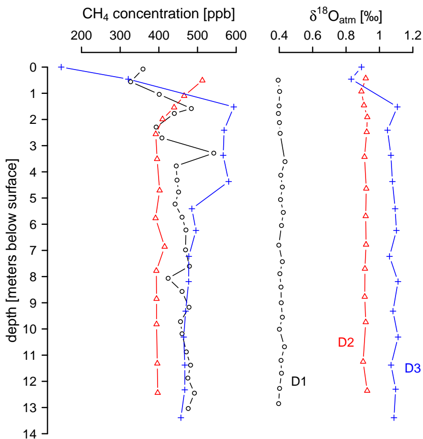
Figure 2. Depth profiles of methane and \delta^{18}\text{O}_{atm} at the sampling sites D1 (○), D2 (△), and D3 (+). The analytical uncertainty based on replicate analyses is smaller than the size of the symbols in the plot for both methane (lab analyses, 1- \sigma of 7 ppb) and \delta^{18}\text{O}_{atm} (1- \sigma of 0.01 ‰)
