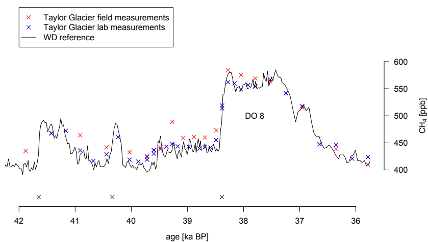
Figure A1. Methane data from Taylor Glacier field analyses (red crosses), lab analyses (blue crosses), and the WD reference record (black line) for a well-sampled time period during MIS 3 including Dansgaard/Oeschger (DO) event 8. Black crosses on the bottom of the plot show fixed tie points used in the WAIS Divide–Taylor Glacier synchronization (Table 1).
