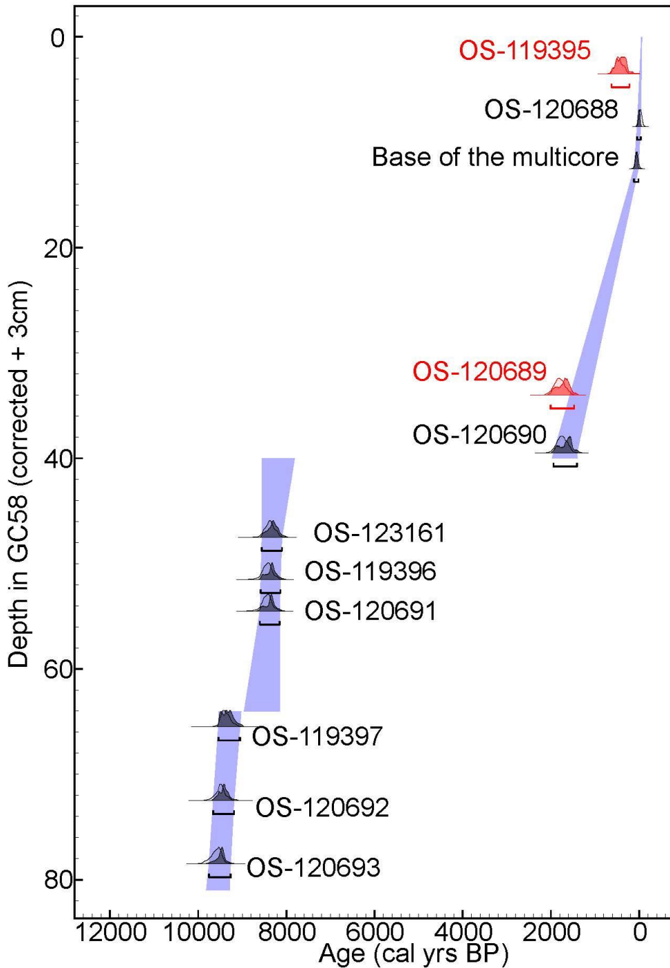
784 785 Figure 2. An age-depth model of the sediment core GC58 based on radiocarbon ( ^{14}\text{C} ) dated molluscs shells (see Table 786 1) and ^{210}\text{Pb} (base of a multicore collected at the same location, see Supplementary Information Table S2). All the 787 modelled dates were calibrated with Marine13 calibration curve (Reimer et al., 2013). A \Delta R value of 50 \pm 100 yrs was 788 used to account for the differences in the local reservoir age based on (Bauch et al., 2001a). The core GC58 dates back 789 \sim 9,500 cal yrs BP. The calibrated age probability distributions are plotted for each radiocarbon date in grey. Outliers
