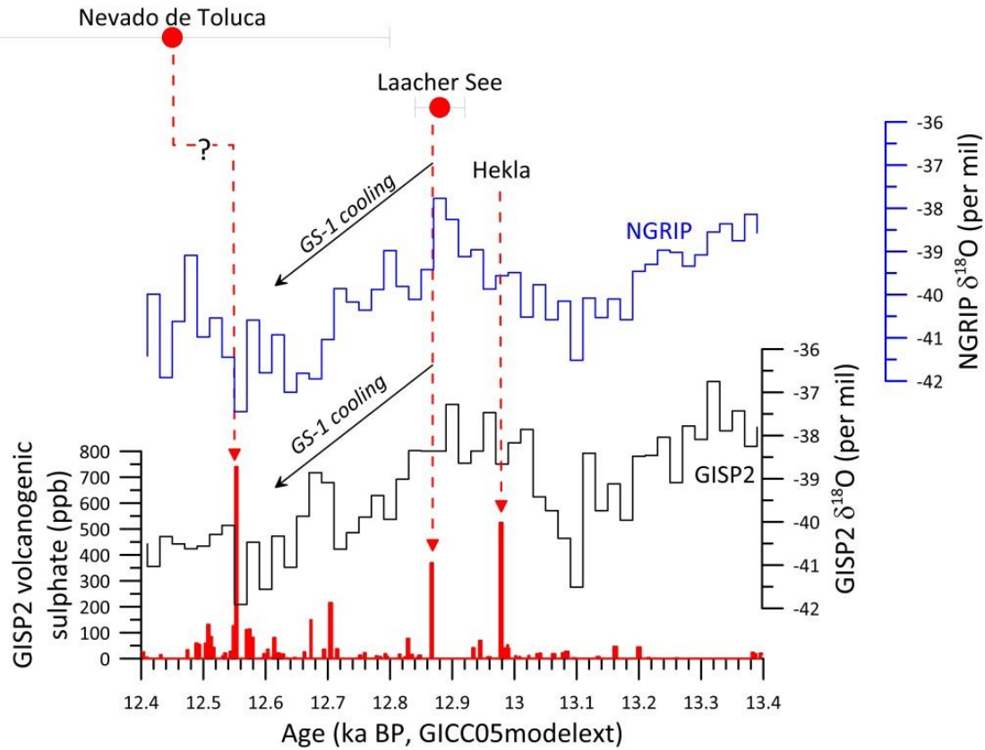
Figure 5. The GISP2 (bidecadal (Stuiver et al., 1995)) (black) and NGRIP (blue) ice core \delta^{18}\text{O} records synchronised on the GICC05modelext chronology (Seierstad et al., 2014). The red bars indicate GISP2 volcanological sulphate record (also synchronised on the GICC05 timescale). The maximum counting error of the ice core chronology is 0.138 ka at 12.9 ka BP (Seierstad et al., 2014). The best age estimate of the LSE is shown (red circle) (Brauer et al., 2008; Lane et al., 2015) and a possible correlation to a synchronous sulphate spike highlighted by the vertical dashed arrow. The large spike at ~13 ka BP represents a smaller but more proximal Icelandic eruption (Hekla) associated with a volcanic ash layer (Mortensen et al., 2005; Bereiter et al., 2018).
