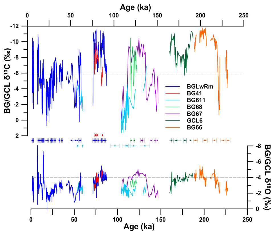
Figure S2. Carbon and oxygen isotopic time series for BG and GCL stalagmites.
