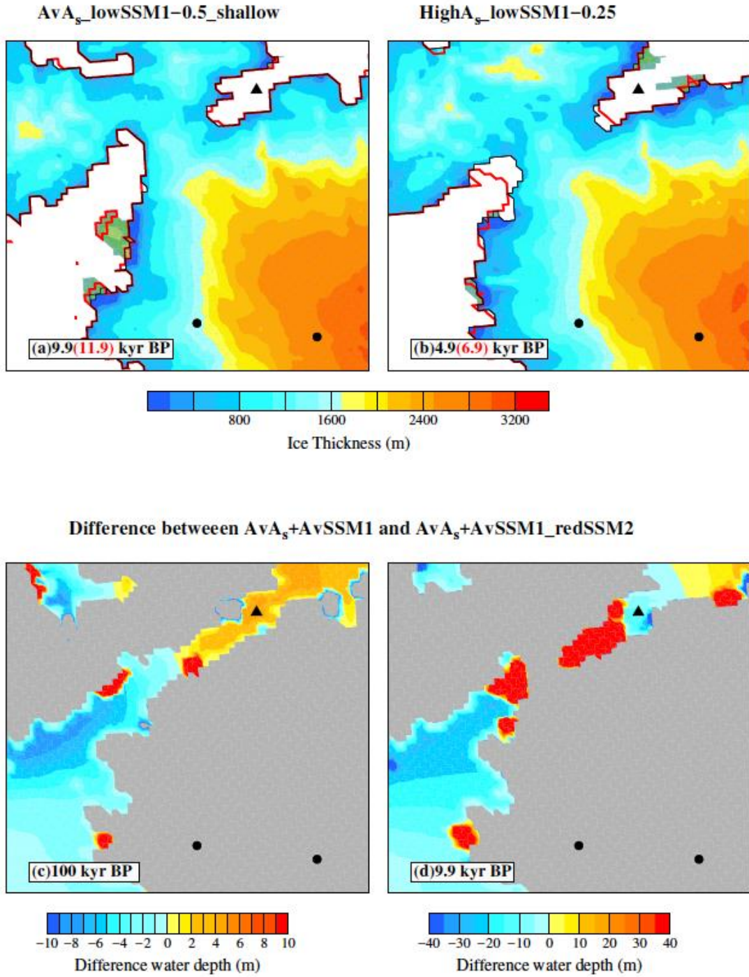
Figure 7: Examples of the influence of the choice of SSM parameter and RSL forcing on the spatial and temporal retreat pattern across the NW margin (yellow box bounded by the blue box on Fig.1). Panels (a) and (b) compare the grounded ice sheet extent in two simulations (AvA s _lowSSM1-0.5_shallow and HighA s _lowSSM1-0.25) to highlight the impact of the choice of A s in controlling the onset of the LGM-PD retreat. The red contour marks the edge of the grounded ice sheet at an earlier time step (given in red). Panels (c) and (d) illustrate the difference in the simulated water depth and maximum grounded ice sheet extent (shaded grey region) between simulations AvA s +AvSSM1 and AvA s +AvSSM1_redSSM2. The main difference between these two simulations is the choice of SSM2: 100 m/yr (AvA s +AvSSM1) compared to 75 m/yr (AvA s +AvSSM1_redSSM2).
