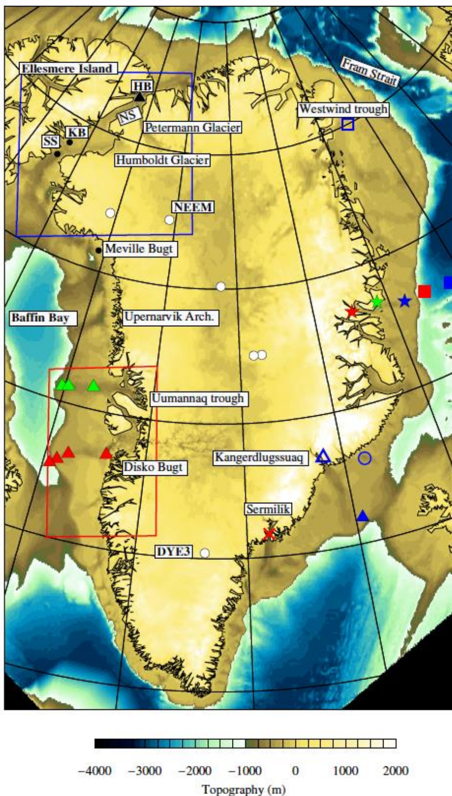
Figure 1: Summary of the main place names and regions referred to in the main text and location of observational data. All information describing the symbols and references for the observational data in listed in Table 1. The red and blue boxes highlight the regions shown on Fig. 6 and Fig. 7 respectively.
