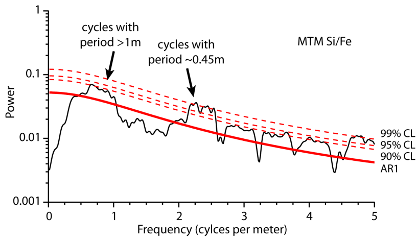
Figure 34. MTM power spectra for Si/Fe ratios; highlighted are spectral peaks equivalent to cycles with period >1 m and ~0.45 m.
