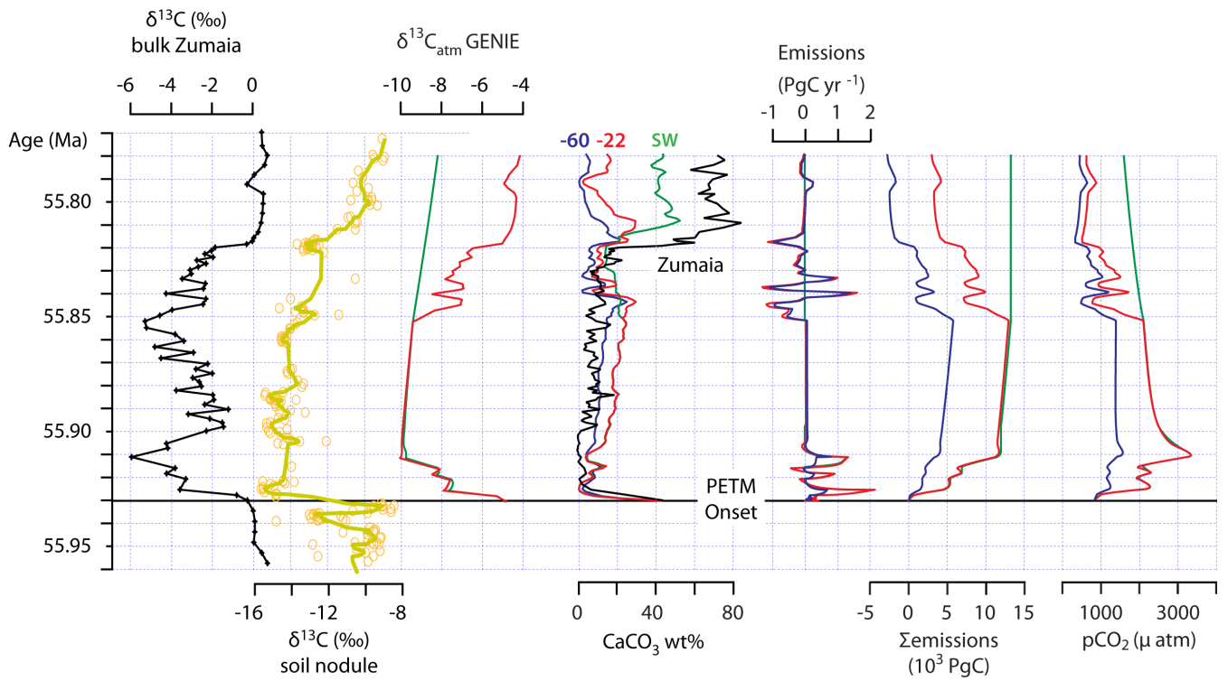
5 Figure 67. Results of inverse modelling with cGENIE Earth System Model. From left to right: the bulk carbonate \delta^{13}\text{C} for Zumaia which drives model inversions (black); soil nodule \delta^{13}\text{C} record of the Big Horn Basin (yellow), as representative of atmospheric \text{CO}_2 \delta^{13}\text{C} for comparison to model results; modelled \delta^{13}\text{C} composition of atmospheric carbon dioxide; carbon emission rate in PgC per year; cumulative carbon emissions (cumulative input minus removal); modelled atmospheric \text{pCO}_2 ; modelled and actual weight % \text{CaCO}_3 content of the sediment column at Zumaia; modelled carbon emission and removal rates; cumulative modelled carbon emissions / removal; modelled atmospheric \text{pCO}_2 . The model scenarios are as follows: 1) carbon input at \delta^{13}\text{C} of -22 ‰ during the onset, no carbon removal (green); 2) carbon input and removal with \delta^{13}\text{C} of -22 ‰ to follow Zumaia target CIE (red); 3) carbon input with \delta^{13}\text{C} of -60 ‰ and removal of carbon with \delta^{13}\text{C} of -22 ‰ to follow Zumaia target CIE (blue). All simulations have active temperature-dependent silicate weathering feedbacks operative throughout. 10
