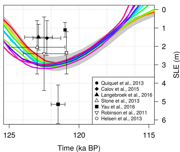
Figure 10. GrIS ice volume evolution simulated for different values of the melting rate sensitivity \kappa during the last interglacial (see Fig. 5 for the line colour legend). The ice volumes have been converted to values of SLE anomaly with respect to the present-day volumes estimated in each specific simulation. Grey shading represents the reference basal melting rates B_{ref} investigated for the case of constant in time oceanic forcing ( \kappa = 0 \text{ m a}^{-1} \text{ K}^{-1} ). Black and white symbols indicate the LIG minimum ice volumes estimated by previous studies. The tight clustering of our estimates compared to previous work is due to the fact that the sole uncertainty is here related to the oceanic forcing through \kappa .
