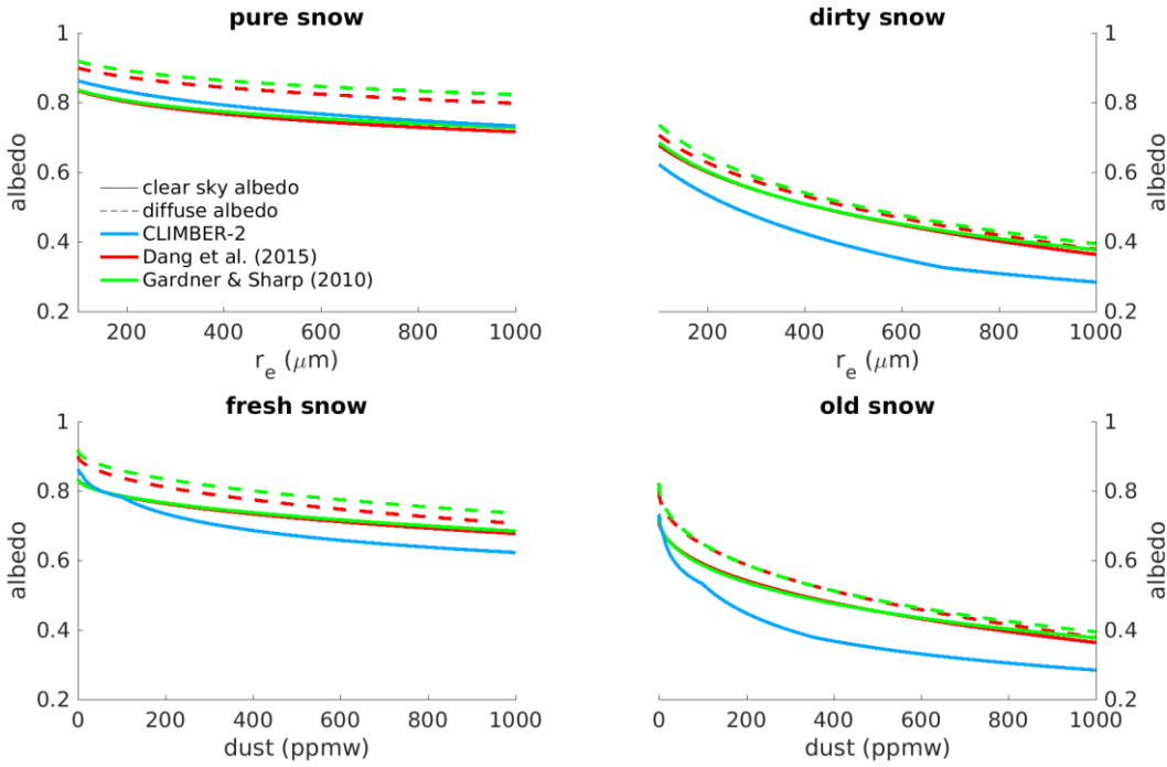
5 Figure 1: Clear sky and diffuse snow albedo dependence for a number of different parameterisations (Dang et al., 2015; Gardner and Sharp, 2010; Warren and Wiscombe, 1980) as indicated in the legend. a) Pure snow albedo dependence on effective snow grain radius. b) Fresh snow albedo ( r_e = 100 \mu\text{m} ) as a function of dust concentration. c) Dirty snow albedo (dust concentration of 1000 ppmw) as a function of snow grain size. d) Old snow albedo ( r_e = 1000 \mu\text{m} ) as a function of dust concentration. The clear sky albedo is for a solar zenith angle of 50^\circ . In CLIMBER-2 the snow albedo for diffuse and direct radiation is identical for solar zenith angles below 60^\circ .
