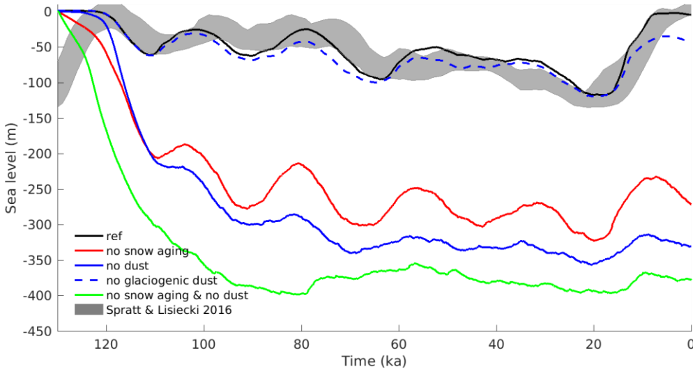
10 Figure 7: Effect of snow aging and dust deposition on modelled sea level over the last glacial cycle for different online experiments as indicated in the legend.
