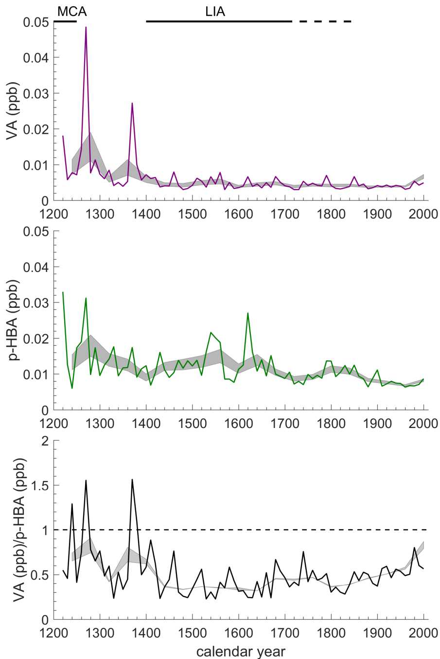
Figure 3. Lomonosovfonna ice core records of vanillic acid (top) and p-hydroxybenzoic acid (middle) and the ratio of vanillic acid/p-hydroxybenzoic acid (bottom). For all plots: solid lines are 10-year bin averages, gray shaded areas are 40-year bin averages of \pm 1 standard error. The dashed line on the bottom plot indicates a ratio of 1. The black horizontal lines are the Medieval Climate Anomaly (MCA) and the Little Ice Age (LIA) (Mann et al., 2009). The dashed horizontal line at the top is the extended LIA in the Svalbard region (Divine et al., 2011).
