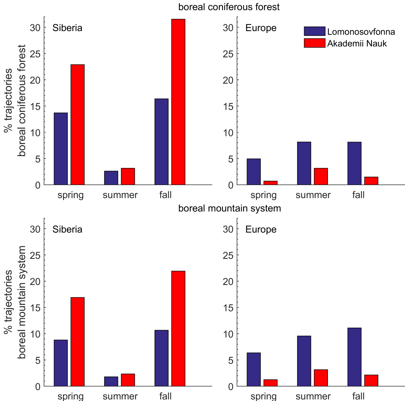
Figure 7. 10-day back trajectories from 2006-2015 reaching the boreal ecosystems starting from the Lomonosovfonna and Akademii Nauk ice core locations. Blue is Lomonosovfonna. Red is Akademii Nauk. Trajectories reaching: Siberia (left), Europe (right), boreal coniferous forest (top), and boreal mountain system (bottom).
