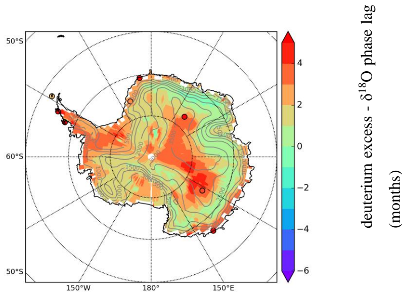
Figure 10: Best correlated phase lag between the mean seasonal cycle of deuterium excess and that of \delta^{18}\text{O} simulated by ECHAM5-wiso over the period 1979-2013 (color shading) and calculated from precipitation data (circles). The sign informs on the sign of the correlation between \delta^{18}\text{O} and d (e.g. positive numbers correspond to a correlation, while negative numbers correspond to an anti-correlation). The absolute value corresponds to the lag (in months) between \delta^{18}\text{O} and deuterium excess corresponding to the highest correlation of monthly averaged values. This figure also displays the Antarctic topography, with isohypses (in m a.s.l.).
