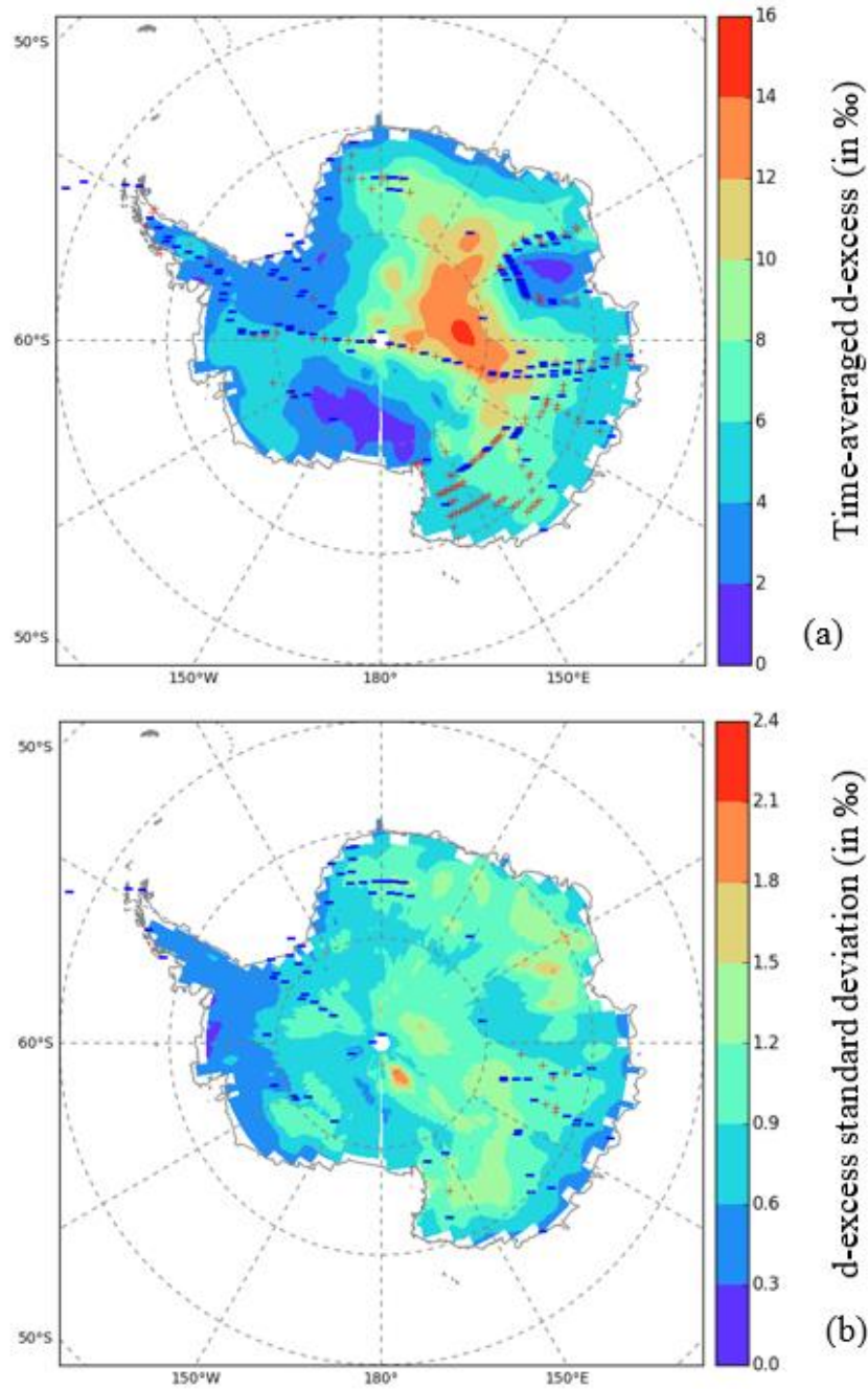
Figure 6: Maps displaying model-data comparisons for d time-averaged (in ‰, a) values and inter-annual standard deviations (in ‰, b). Backgrounds correspond to ECHAM5-wiso simulations over the period 1979-2013, while signs correspond to the model-data comparison. For the time-averaged values, the comparison consists in calculating the model-data differences. Red “+” symbols indicate a positive model-data difference while blue “-” symbol correspond to a negative model-data difference. For the inter-annual standard deviation, the comparison consists in calculating the ratio of the simulated value to the corresponding grid point data. Red “+” symbols indicate a ratio higher than 1 while blue “-” symbol correspond to a model/data ratio lower than 1.
