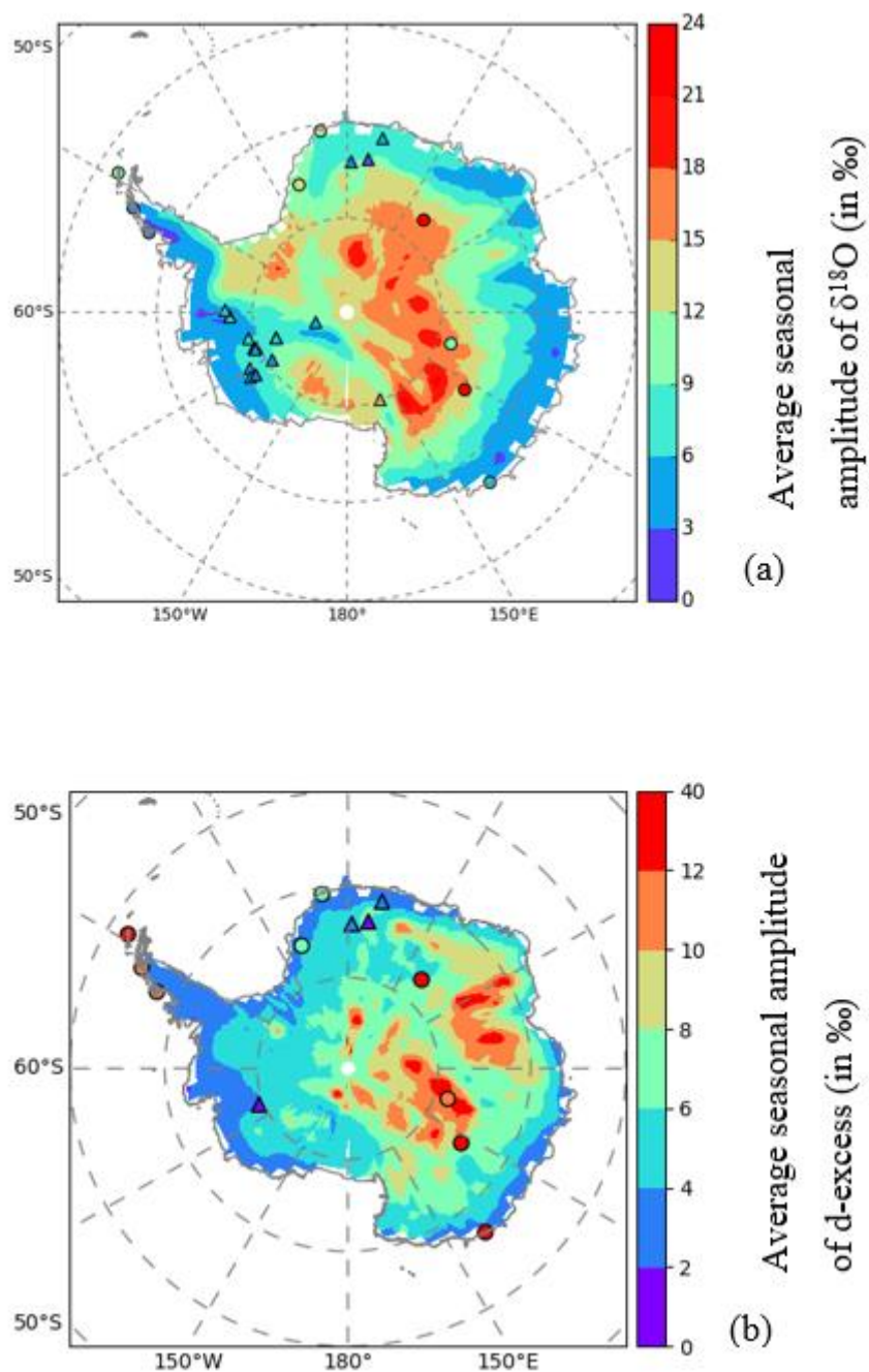
Figure 7: Average seasonal amplitude of precipitation \delta^{18}\text{O} (a) and d (b) (in ‰) simulated by ECHAM5-wiso (color shading) over the period 1979-2013 and calculated from precipitation data (circles) and ice core records (triangles) over their respective available periods.
