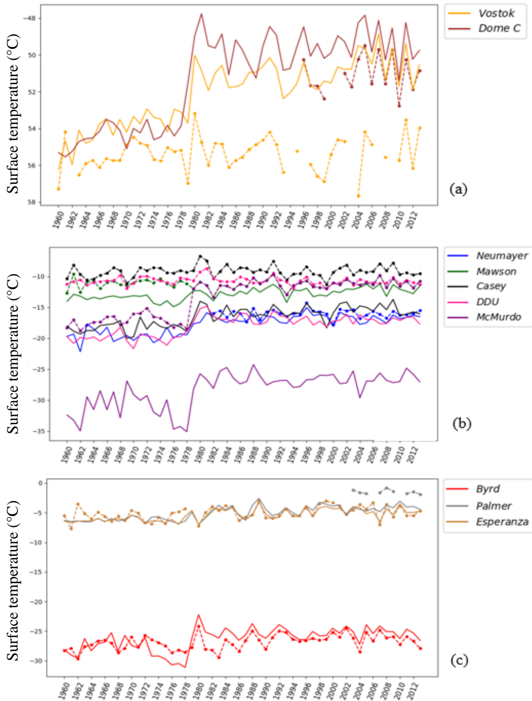
Figure 2: Surface air temperature (in °C) from station instrumental records (points and dashed lines) and simulated by the ECHAM5-iso model (solid lines) over the period 1960-2013 for (a) the Plateau, (b) Coastal East Antarctic Ice Sheet and (c) the West Antarctic Ice Sheet. Note that the plots were organized by regions to make it more readable: inland (a), coastal (b) and West Antarctic Ice Sheet plus Peninsula (c).
