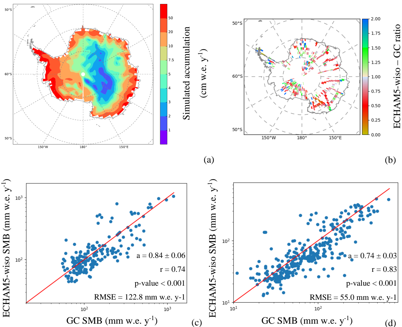
Figure 4: Comparison of the Glacioclim (hereafter, and noted in the plots “GC”) SMB database averaged within the ECHAM5-wiso grid cells and the SMB (i.e. precipitation – evaporation) simulated by the model, with first the spatial distribution of the accumulation (a) as simulated by the model (in cm w.e. y -1 ), (b) the ratio of the ECHAM5-wiso annual accumulation (precipitation minus evaporation) to the GC averaged SMB (no unit), and finally GC averaged SMB values against SMB values simulated by the model (blue dots) associated with the corresponding linear relationships (red solid line), displayed at the logarithm scale, for elevation ranges of 0-2200 m a.s.l. (with the upper limit excluded) (c) and 2200-4000 m a.s.l. (d).
