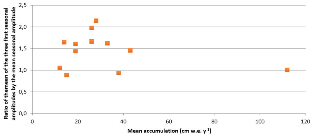
Fig. 1 : Ratio of the three first seasonal amplitude average by the mean seasonal amplitude in function of the mean accumulation
