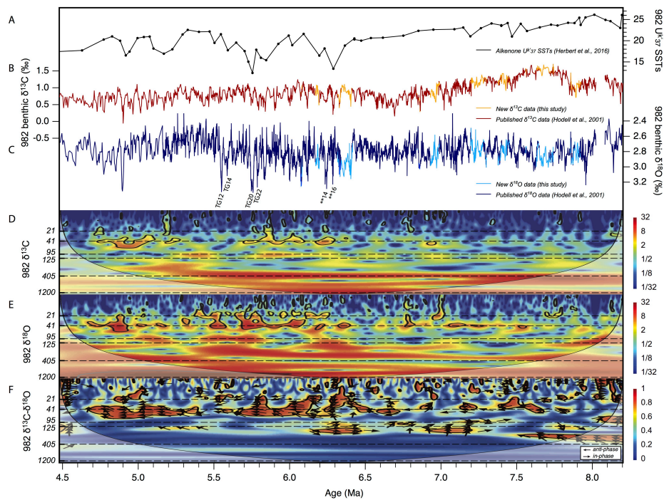
Figure 7: A Alkenone U^k_{37} -derived SSTs from Site 982 (Herbert et al., 2016). B Fine-tuned Site 982 benthic foraminiferal \delta^{13}C (in ‰ versus VPDB). C Fine-tuned Site 982 benthic foraminiferal \delta^{18}O (in ‰ versus VPDB). D Wavelet analysis of the Site 982 benthic \delta^{13}C data (in ‰ versus VPDB) on the fine tuned astrochronology. E Wavelet analysis of the Site 982 benthic \delta^{18}O data (in ‰ versus VPDB) on the fine tuned astrochronology. F Coherence wavelet analysis of the Site 982 benthic \delta^{13}C and \delta^{18}O , with the black arrows to the left indicating anti-phase and the black arrows to the right indicating in-phase. Prominent MIS are annotated, with ** standing for C3An. \delta^{18}O . All wavelets were generated using (Grinsted et al., 2004).
