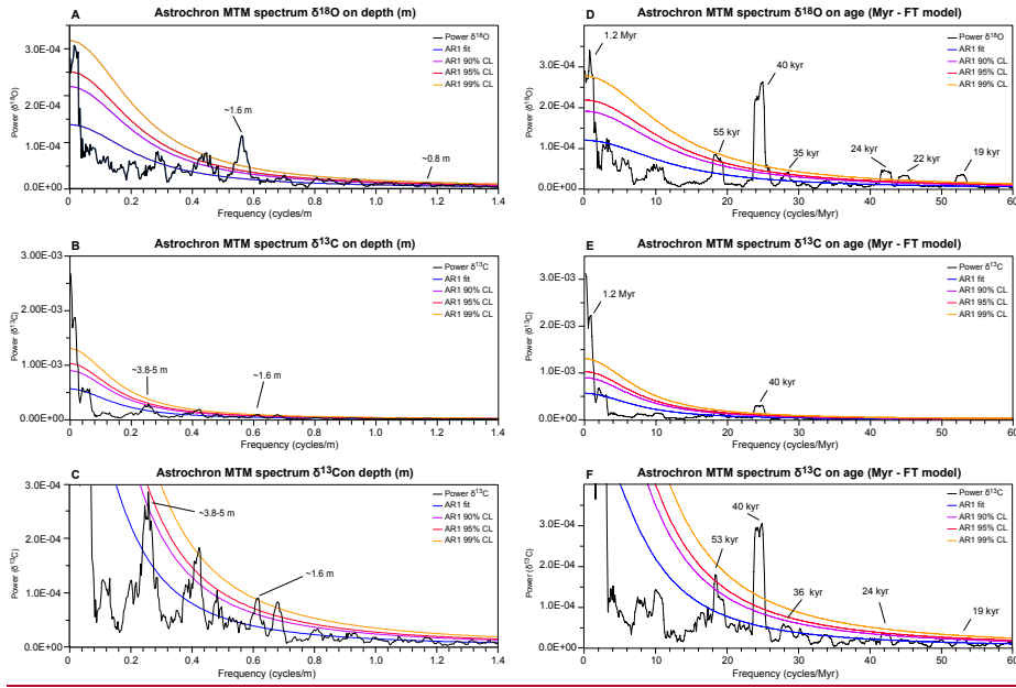
Figure 5: Multitaper method (MTM) power spectra generated using Astrochron (Mevers, 2014; for the specific code, please see the Supplementary Information) for \delta^{18}\text{O} in A/D) and \delta^{13}\text{C} with a full vertical axis shown in B/E) and vertically expanded in C/F to show the same vertical axis extent as in A/D). The red noise fit (AR1) and 90, 95 and 99% confidence limits (CL) relative to red noise are also indicated. The periods of different peaks are annotated. The MTM spectra are shown in the depth domain in A), B) and C) and in the time domain in D) E) and F).
