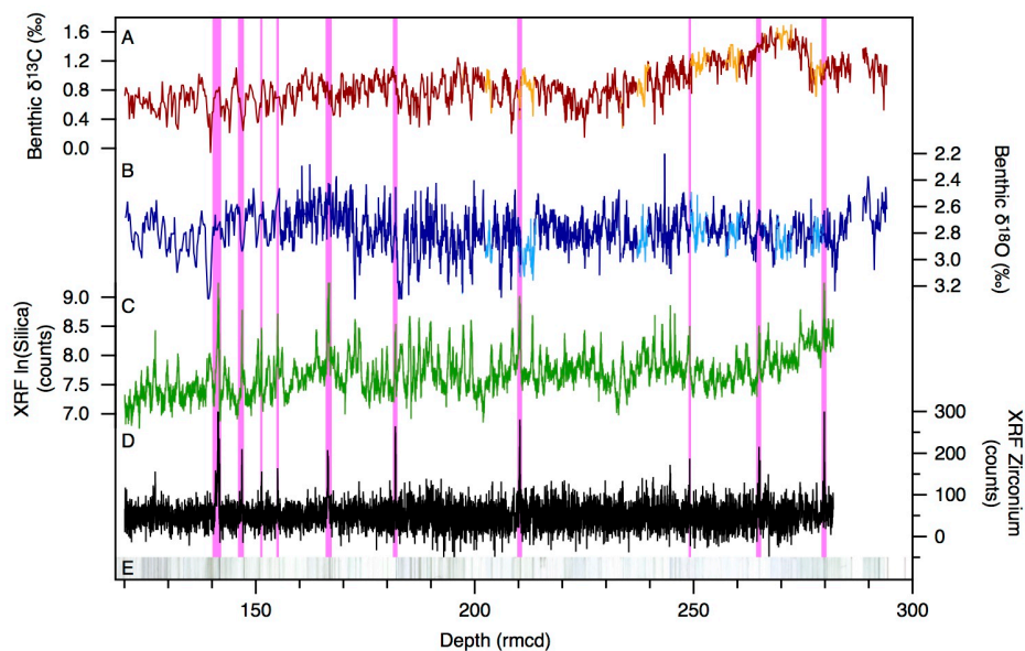
Figure 4: Overview of the new XRF and updated stable isotope datasets on the revised composite depth at Site 982. The complete benthic \delta^{13}\text{C} records from this study (orange) and Hodell et al. (2001) (red) and \delta^{18}\text{O} records from this study (light blue) and Hodell et al. (2001) (dark blue), the XRF counts for \text{In}(\text{Silica}) (green) and \text{Zr} (black), and \text{E} the composite splice image for Site 982. Pink intervals highlight the location of ash layers, based on the presence of Zr peaks, which affect the XRF data, but show no influence on the stable isotope records.
