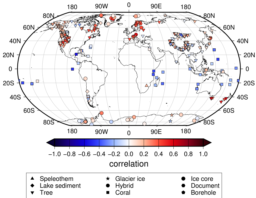
Figure 1. Point-wise correlation between the raw proxy series in the PAGES-SEL network and the SAT in the infilled HadCRUT4 dataset during the period 1911-1995. Each type of proxy is indicated with a different symbol.
