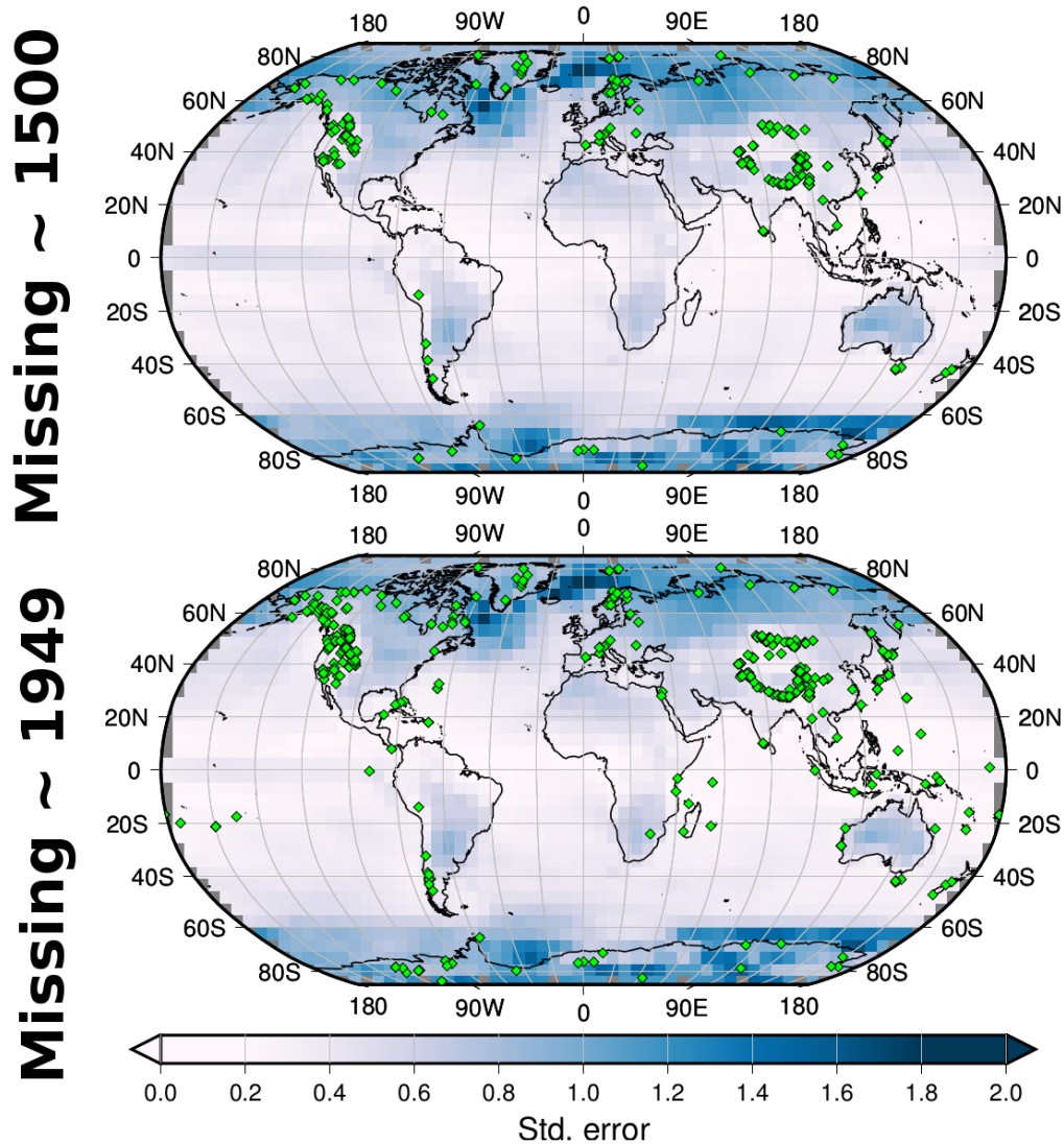
Figure 11. Local standard deviation of the residuals (GISS rli1p1 annual mean SAT minus pseudo-reconstructed SAT) over the period 1850-2005. Top: using a pseudo-proxy network with as many missing values as the PAGES-SEL network in 1500 (257 records). Bottom: using the maximum number of pseudo-proxy locations of the same network, which happens in 1949 (514 records). The precise location of the pseudo-proxies is indicated with green symbols.
