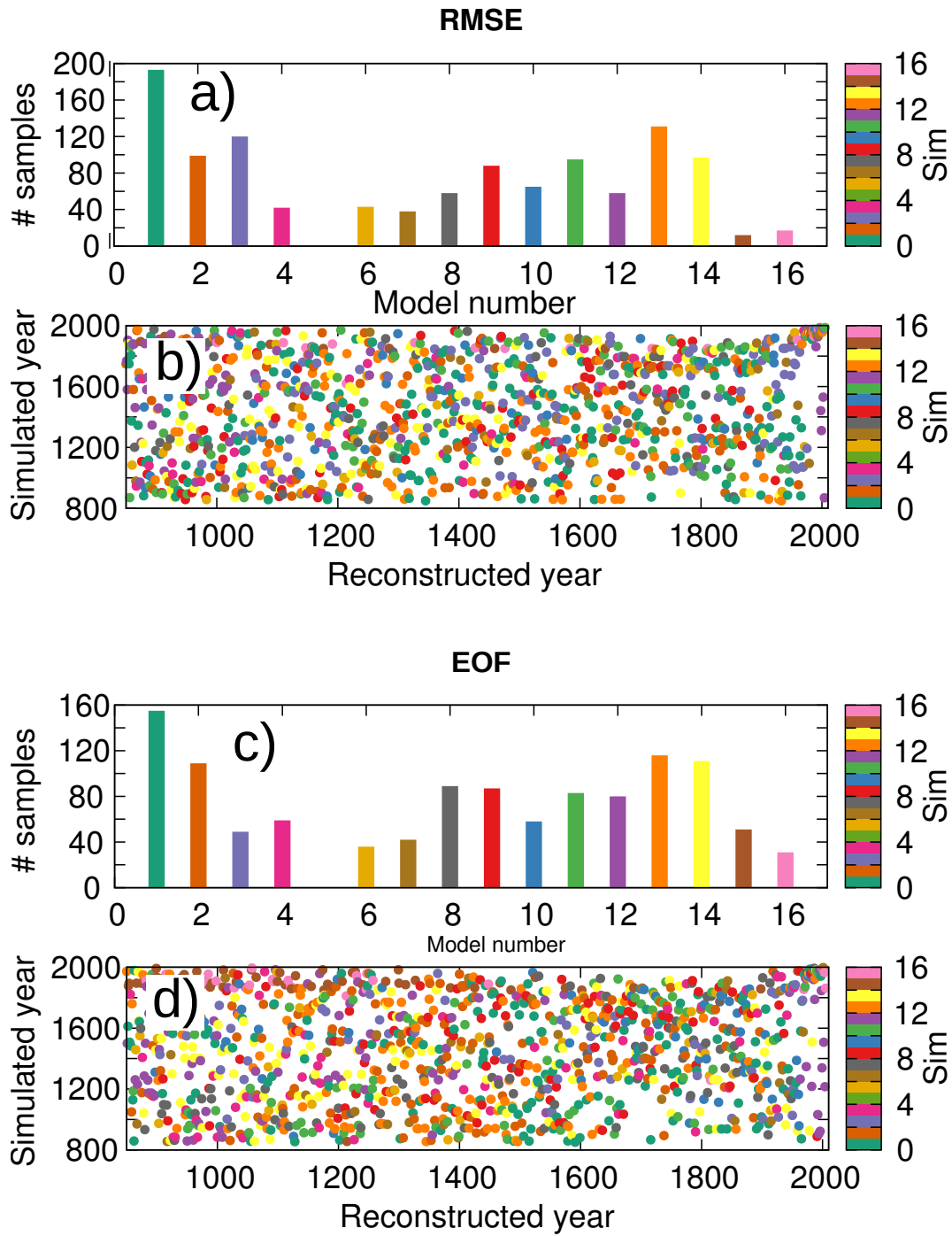
Figure 4. Selection of analogs used to carry out a perfect PPE. Bars in panels a and c indicate the number of times the analog has been taken from each of the 16 models. The points in panels b and d indicate the relationship between the reconstructed year (x-axis) and the model (colour) and simulated year (y-axis) used as analog for the reconstruction. a and b correspond to the reconstruction based on RMSE and c and d based on Euclidian distance in the EOF space.
