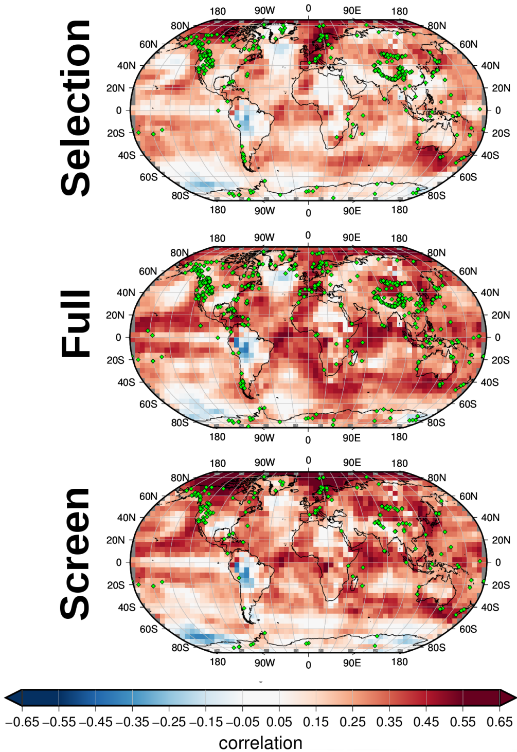
Figure 9. Correlation maps similar to Fig. 8 for the RMSE-AM variant of the AM method. The three maps depict the result obtained using each of the three variants of the PAGES2K network described in Section 2.2. In all cases the green symbols indicate the location of the proxies employed to reconstruct.
