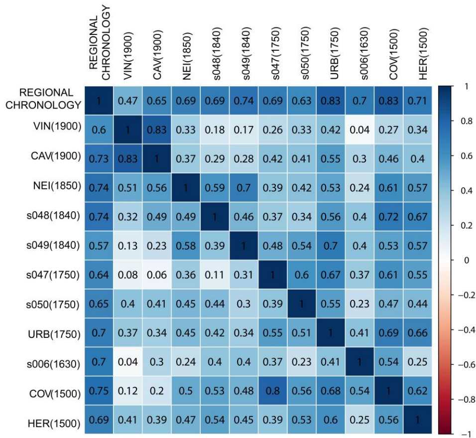
Figure 3. Inter correlation of the raw chronologies between sites and the regional chronology, sorted by elevation. Top right shows the correlations calculated over the common period
