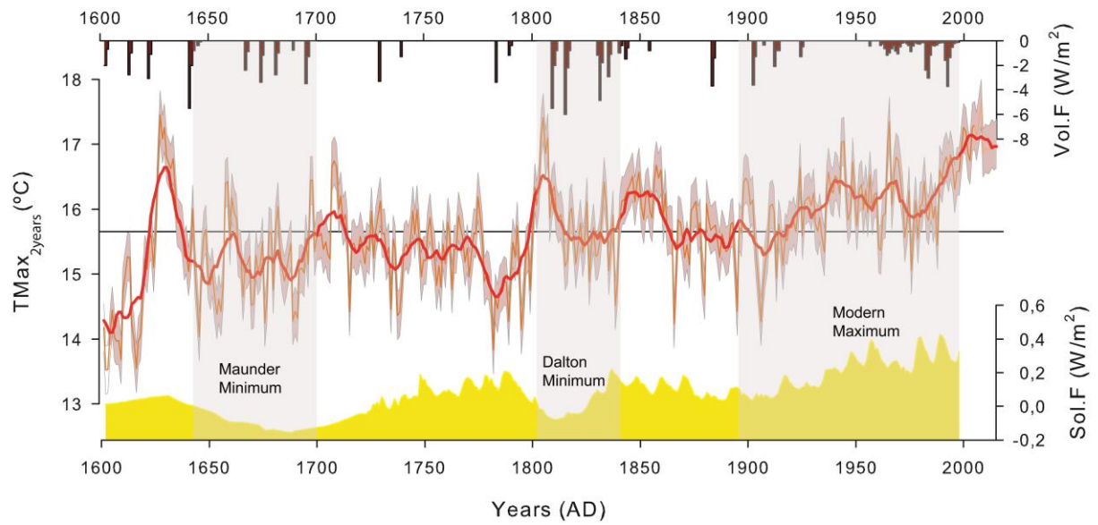
Figure 9. IR2T max reconstruction since AD 1602 for the Iberian Range. Bold red curve is a 11-year running mean, purple shading indicates the mean square error based on the calibration period correlation. Yellow shading at the bottom show solar forcing and bars on top indicate volcanic forcings (Crowley 2000).
