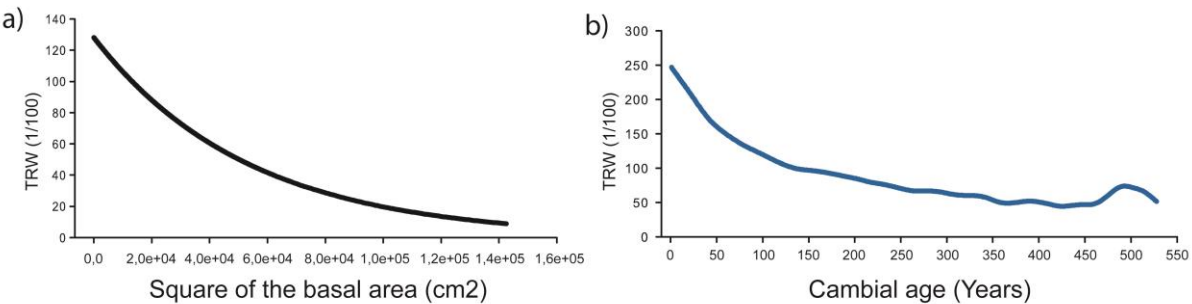
Figure 4. a) Represents the model of the BasPois method, b) represents the regional curve of the RCS method.
