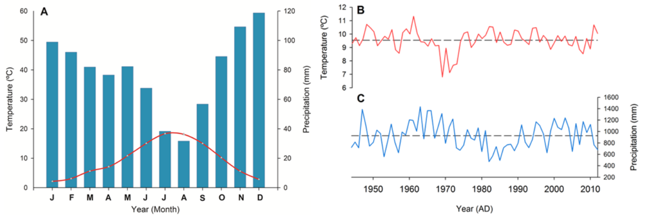
Figure 2. Climate diagram (A), mean temperature (B), mean precipitation (C) calculated using data from CRU TS v.3.22 over the period 1944-2012 (Harris et al 2014).
