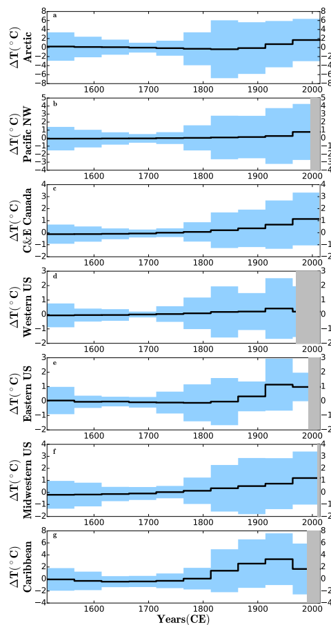
Fig. 3. Mean ground surface temperature histories for seven climate-differentiated regions in North America.
