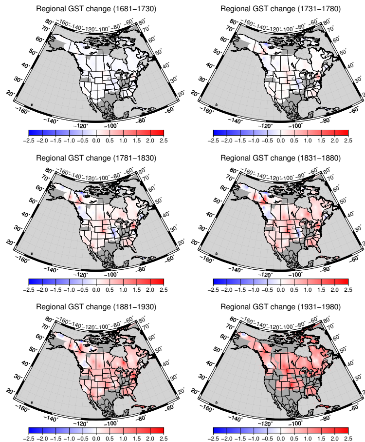
Fig. 4. Spatial variability of the ground surface temperature variation from 1681 to 1980.
