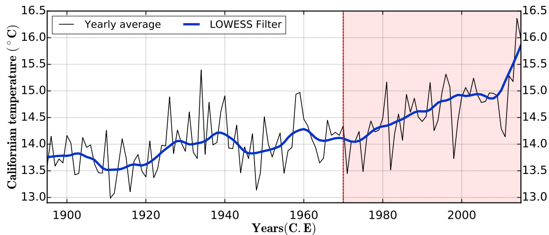
Fig. 2. NOAA's annual mean temperature of California since 1895.
