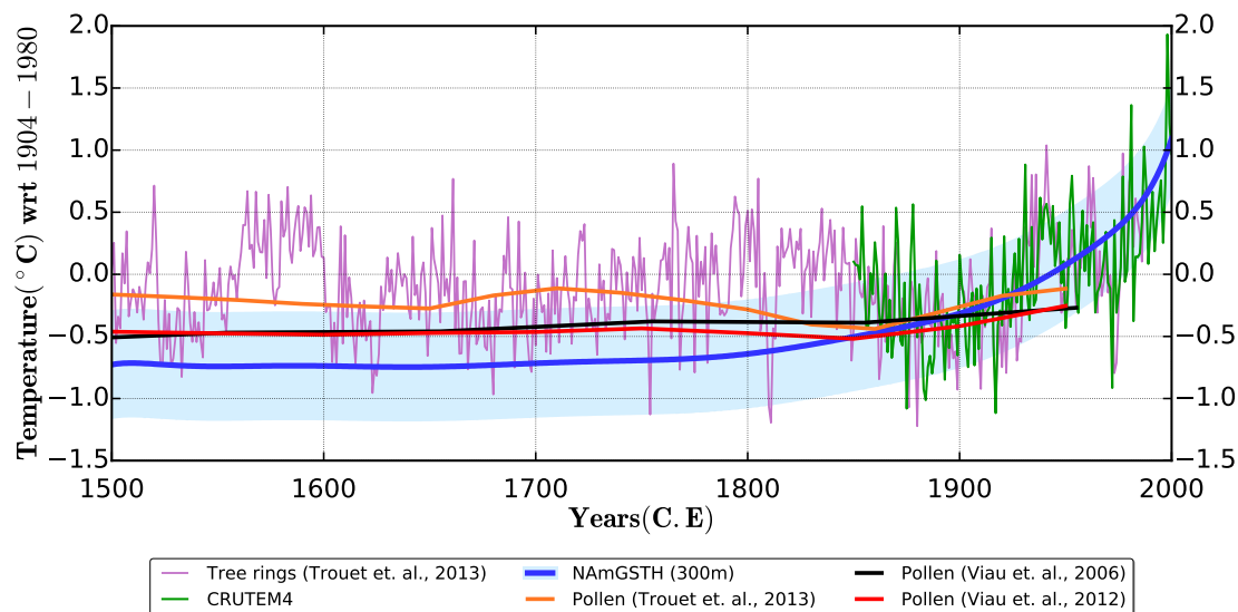
Fig. 1. Comparison of mean North American ground surface temperature history with other proxy reconstructions.
