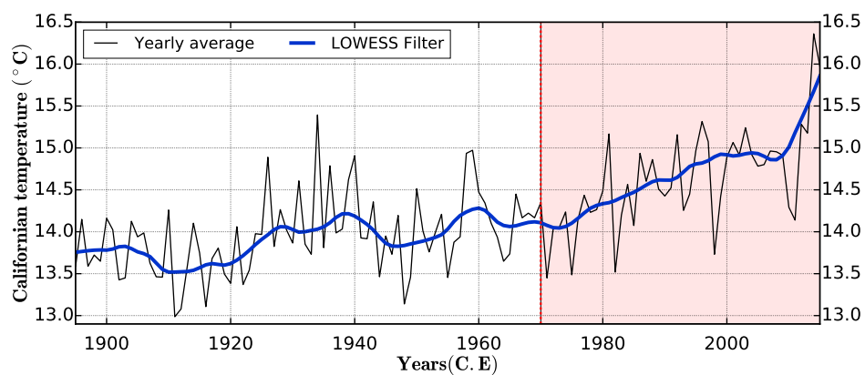
Fig. 2. NOAA's annual mean temperature of California since 1895.
