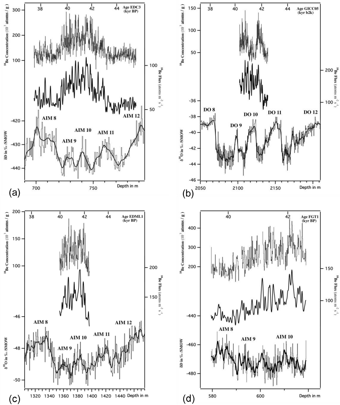
5 Figure 1: ^{10}\text{Be} concentrations, ^{10}\text{Be} flux and stable isotope profiles ( \delta\text{D} or \delta^{18}\text{O} ) and their running averages as a function of depth and age in 4 ice cores a) EPICA Dome C; EDC3 timescale (Parrenin et al., 2007), b) NGRIP; GICC05 timescale (Andersen et al., 2006), c) EDML; EDML1 timescale (Ruth et al., 2007), and d) Vostok: FGT1 timescale (Parrenin et al., 2004). The ^{10}\text{Be} flux has been calculated using accumulation rates used in the above timescales and smoothed with a 50 year binomial filter. AIM stands for Antarctic Isotope Maximum.
