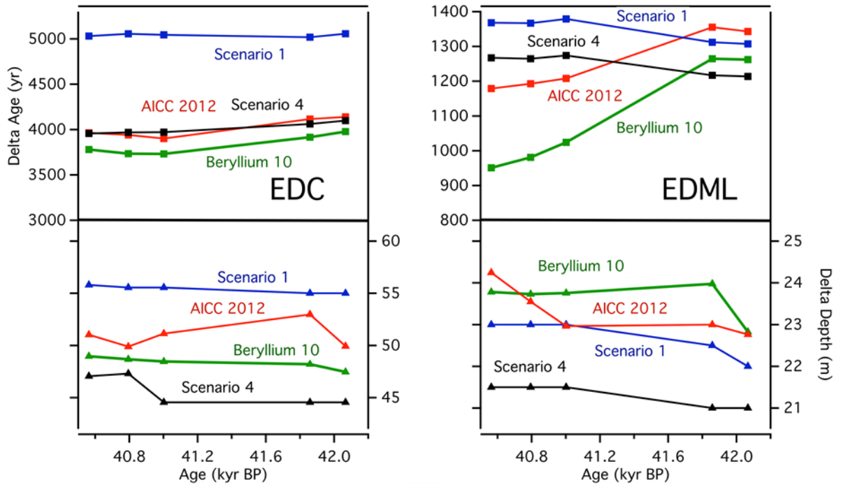
Figure 5: \Delta age and \Delta depth derived for the 5 beryllium-10 tie points derived in this work compared with their values as used in scenario 1 and 4 (Louergue et al., 2007) and for AICC2012 (Bazin et al., 2013).
