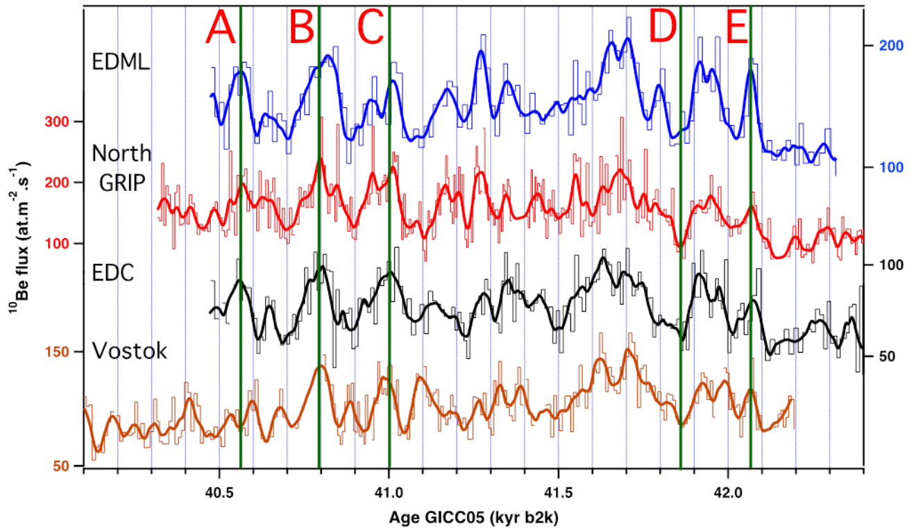
Figure 2: Beryllium 10 fluxes after synchronisation to NGRIP (GICC05) using Match protocol (Lisiecki and Lisiecki, 2002) for EDC and EDML, or using 5 tie-points (A-E) and Analysieries (Paillard et al., 1996) for Vostok. For each site the detailed fluxes (histograms calculated using 11 cm accumulation rates for NGRIP, 55 cm for EDC, 50 cm for EDML and 10 cm for Vostok) and results smoothed with a 50 year binomial filter (curve) are shown.
