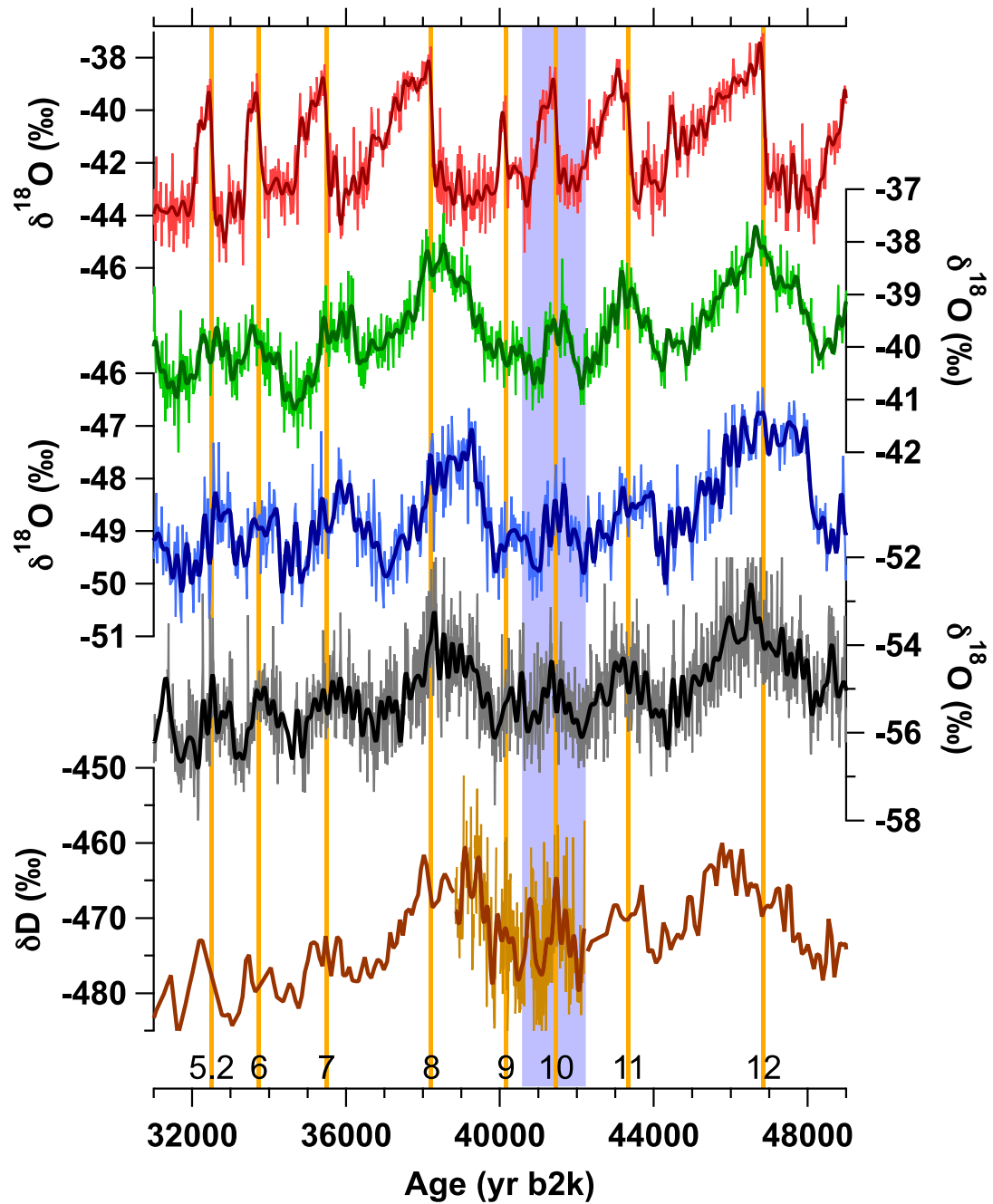
Figure 7: Water isotopic records for NGRIP and 4 Antarctic ice cores over DO events 5 to 12 on the GICC05 timescale with the transition between GS and GIS indicated by the vertical orange lines. The synchronization between NGRIP (red), EDML (blue), EDC (black) and Vostok (brown) is based on the AICC2012 timescale while the WDC (green) record has been transferred on the GICC05 timescale as WD2014 in Buizert et al. (2015).
