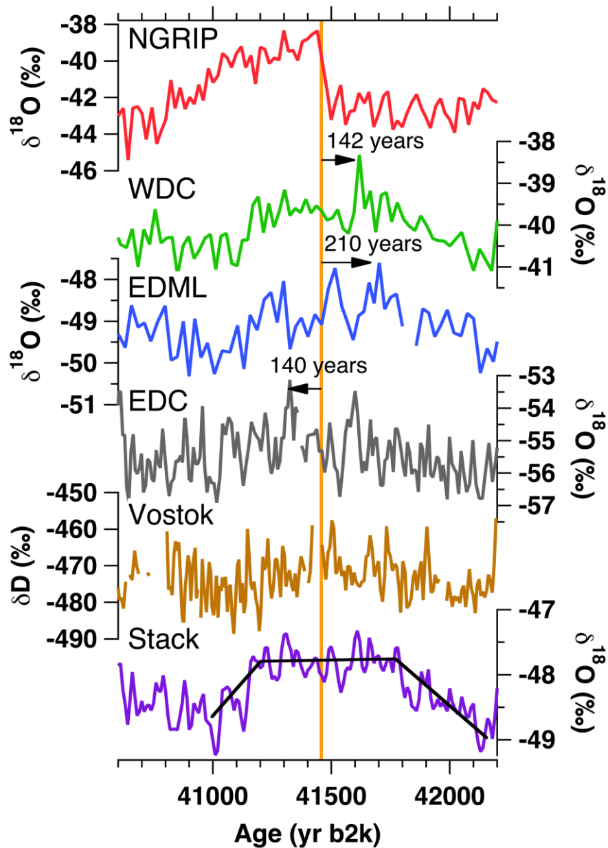
5 Figure 8: Phasing between the GS-GIS transition in Greenland (vertical orange line) and the maximum of the AIM 10 in 4 different Antarctic ice cores on the GICC05 age scale. The synchronicity between Vostok, EDC, EDML and NGRIP is based on the ^{10}\text{Be} records while the WDC isotopic record has been drawn on the GICC05 timescale using the correspondence between the WSD timescale and GICC05 given in Buizert et al. (2015). A stack (purple curve) is drawn using the 3 \delta^{18}\text{O} records from EDML, EDC and WDC, and the black lines correspond to its inflexions identified by eye.
