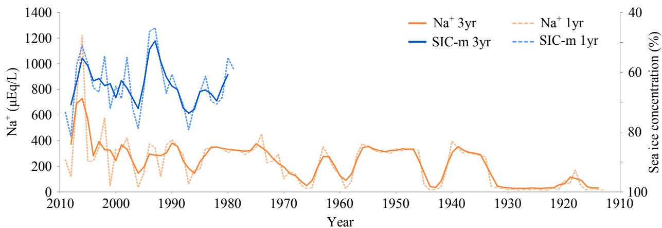
Figure 10. Time series of mean SIC-m (blue, right y axis) and, \text{Na}^+ (orange, left y-axis) over the period from 1913 to 2009. Note that the right y axis is reversed to highlight the high degree of anti-correlation.
