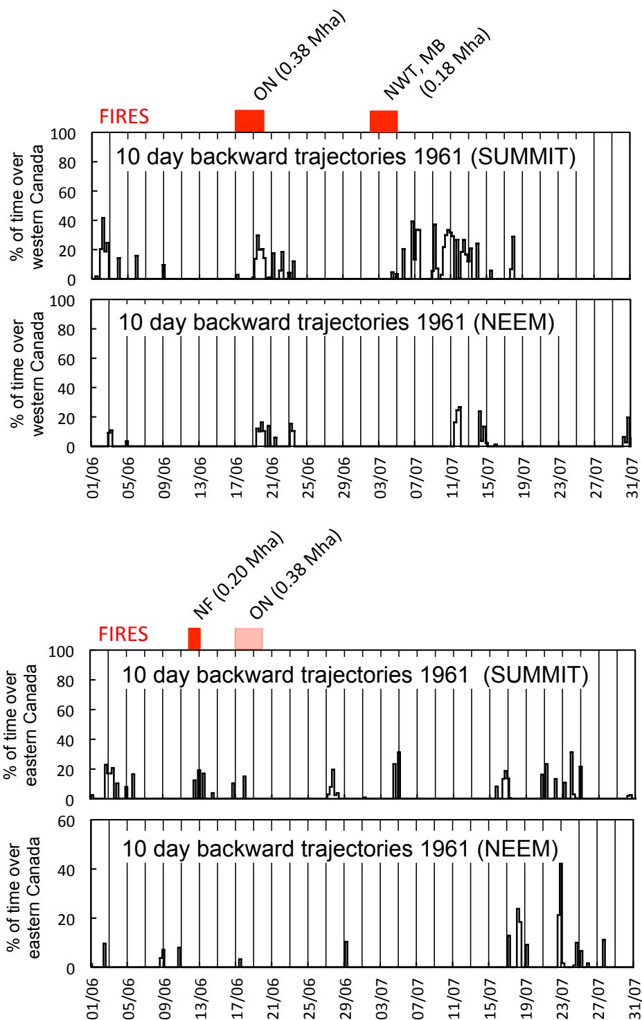
5 Figure 12: Fraction of time spent by air masses arriving at Summit and NEEM (ten-day backward trajectories) at 500 m agl and having traveled over a forested area of western (top) and eastern (bottom) provinces of Canada during the severe fire conditions of June/July 1961 (Fig. 10). Some of the largest fires are indicated on top of the panels (red symbols) with corresponding burned area: Ontario and Northwest Territories in the West, Newfoundland and Labrador in the East. The Ontario fire was located in the western portion of the province and we report the red symbol on both panels. Area burned data are from the Canadian National fire database (Sect. 4.1.1).
