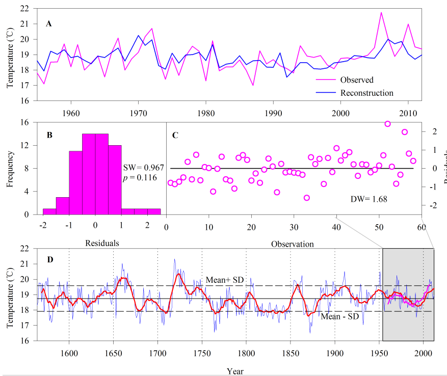
Fig. 7. Temperature reconstruction in NWSP, China. A, The comparison of observed (pink line) and reconstructed (blue line) regional Jul-Aug mean maximum temperature during the calibration period 1955-2012; B,
