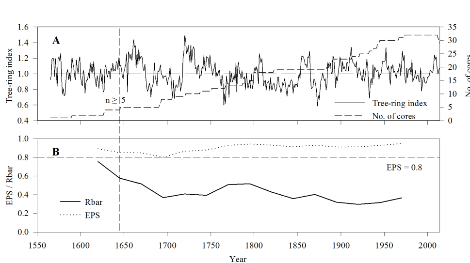
Fig. 1. The tree-ring chronology of Picea purpurea at timberline in Chali. A, Standard chronology and sample size changing with time and B, Rbar and EPS (see text for explanation) plotted for 50-year windows
