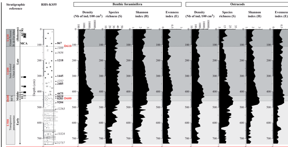
Figure 6: Ecological indices (total abundance per 100 cm 3 , number of species (S), Shannon (H) and Evenness (E) index) describing benthic foraminiferal and ostracod populations. Correlations with seismic units and Holocene cooling events are shown on the left side of the figure discontinuities are shown on the left side of the figure. The corresponding positions of seismic units and discontinuities (U500, U600, U610, D600 and D610) are also reported on the plots (grey bands and dashed lines). Black rectangles on the left side of the figure represent the most significant periods of climate deterioration (i.e. Cold Relapses (CRs)) during the Holocene.
