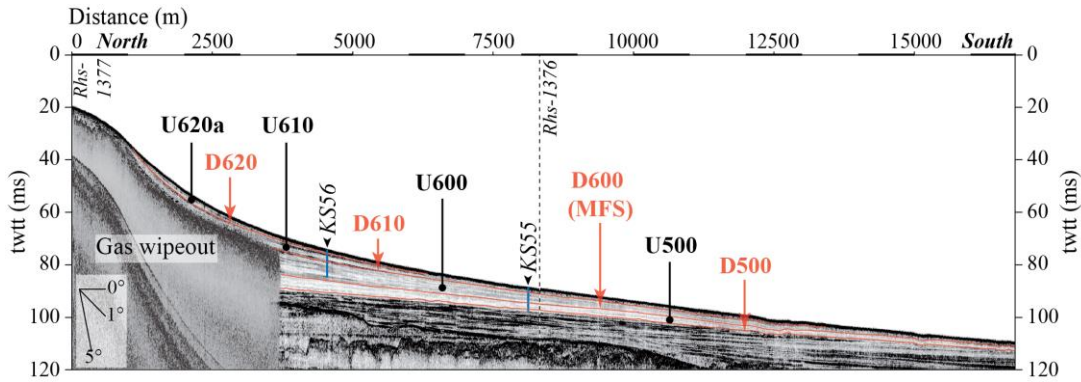
Figure 2: "Dip" (NS) chirp seismic profile across the Grand Passon and Bras de Fer subaqueous delta (position in Fig. 1). Surface D500 corresponds to the flooding surface (that coincides here with a wave ravinement surface) that separates the Younger Dryas (seismic unit U400) deposits from the Preboreal deposits (seismic unit U500). The downlap surface D600 is the Maximum Flooding Surface formed during the turnaround between retrogradation and progradation. D610 and D620 are erosional surfaces that mimic flooding surfaces and separate the middle and late Holocene sedimentary wedges (seismic units U600, U610 and U620a) formed in response to the successive shifts of Rhone Channel.
