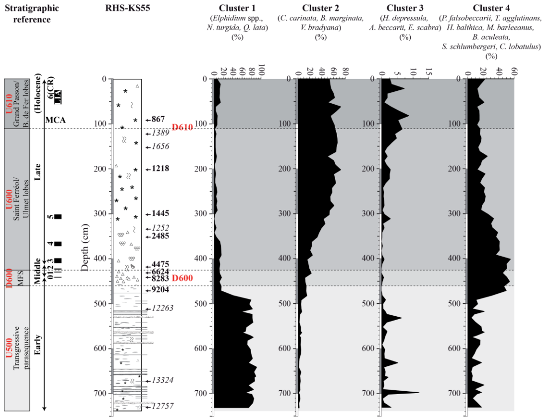
890 Figure 9: Cumulative percentages of taxa composing the defined benthic foraminiferal clusters along core RHS-KS55. Correlations with seismic units and Holocene cooling events are shown on the left side of the figure, discontinuities are shown on the left side of the figure. The corresponding positions of seismic units and discontinuities (U500, U600, U610, D600 and D610) are also reported on the plots (grey bands and dashed lines). Holocene Cold Relapses (CRs) are also indicated on the y-axis by the black rectangles (left side of the figure). 895
