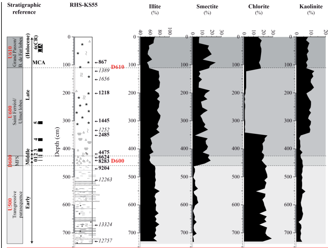
Figure 5: Distribution of the main clay minerals in core RHS-KS55. Correlations with seismic units and Holocene cooling events are shown on the left side of the figure, discontinuities are shown on the left side of the figure. The corresponding positions of seismic units and discontinuities (U500, U600, U610, D600 and D610) are also reported on the plots (grey bands and dashed lines). Black rectangles on the left side of the figure represent the most significant periods of climate deterioration (i.e. Cold Relapses (CRs)) during the Holocene.
