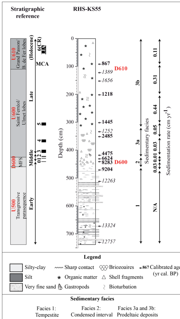
Figure 4: Sediment features and sedimentation rates of core RHS-KS55. Correlations with seismic units and discontinuities and with the Holocene chronology are shown— Black rectangles on the left side of the figure. Black rectangles represent the most significant periods of climate deterioration (known as Cold Relapses (CRs), Wanner et al., 2014) during the Holocene (e.g. the 8.2 ka event and the Little Ice Age ), (CR0) and the Little Ice Age (CR6) ). AMS 14 C dates are mentioned to the right; italic values correspond to age inversions . 14 C dates are summarized in Table 2 .
