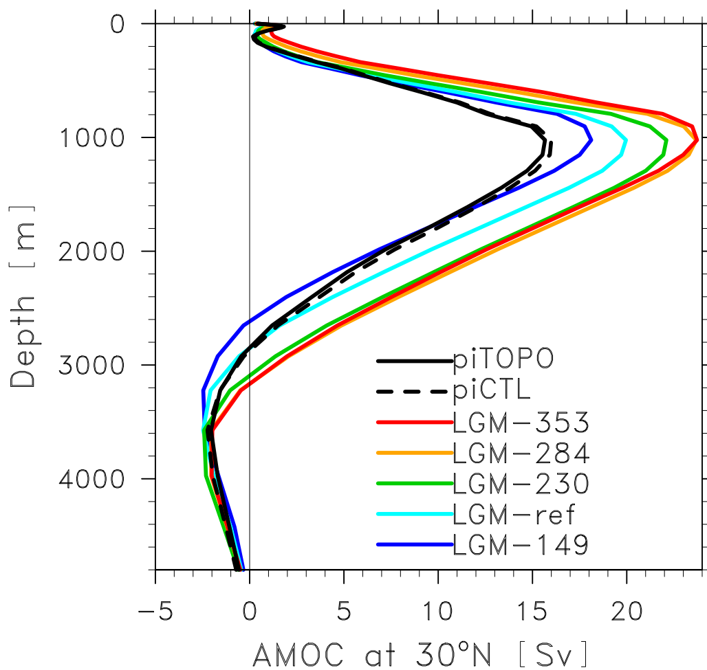
Figure 7. Profile of the AMOC at 30°N for the different experiments. Experiments with LGM setup are shown in color, experiments with piTOPO setup are shown in black and gray.
