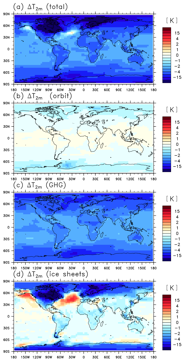
Figure 1. 2m air temperature differences in response to (a) the total glacial forcing (LGM-ref – piCTL), (b) the orbital configuration (piTOPO – piCTL), (c) the glacial GHG concentrations (LGM-ref – LGM-284) and (d) the ice sheets (LGM-284 – piTOPO).
