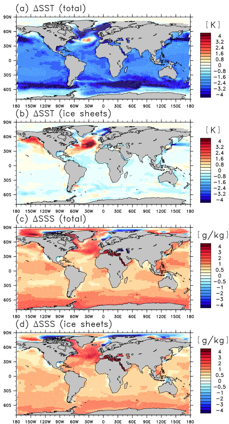
Figure 3. (a) SST response to the total glacial forcing (LGM-ref – piCTL) (b) SST response to the ice-sheets (LGM-ref – LGM-284), (c) sea surface salinity (SSS) response to the combined glacial forcings (LGM-ref – piCTL) and (d) SSS response to the ice sheets (LGM-ref – LGM-284).
