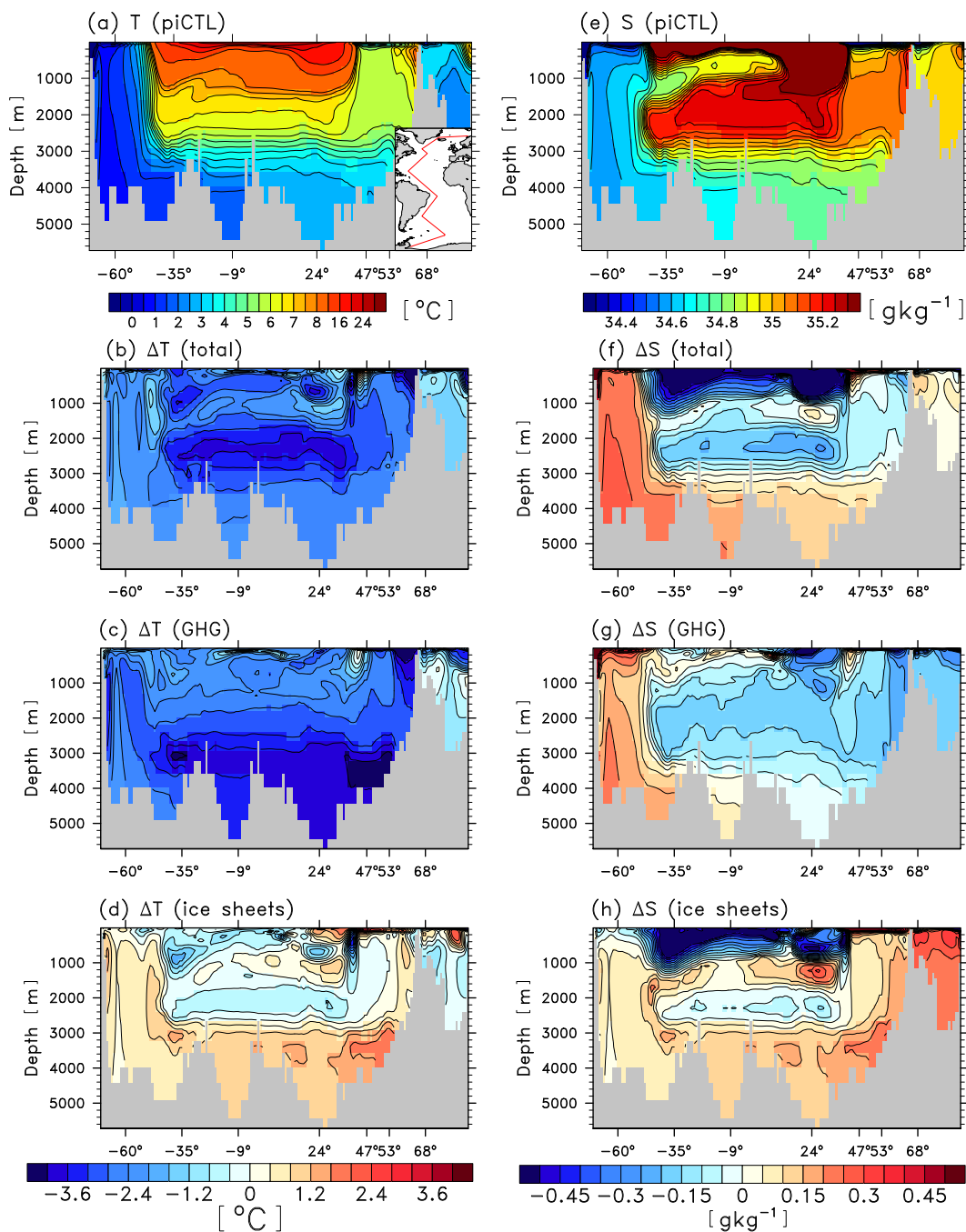
Figure 5. Transect through the Atlantic. (a-d) From top to bottom: potential temperature in piCTL and temperature changes due to the total glacial forcing (LGM-ref – piCTL), the glacial GHG concentrations (LGM-ref – LGM-284) and the ice sheets (LGM-284 – piTOPO). (e-h) As left column but for salinity. Before calculating the differences, the salinity of piCTL and piTOPO has been increased by 1.21 g kg -1 for comparison with the GHG induced differences (LGM-ref – LGM-284). A map of the transect is shown in the top left panel.
