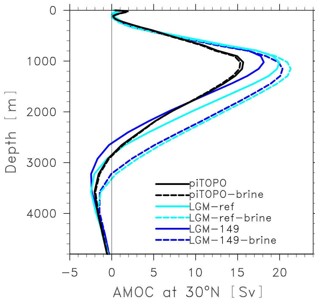
Figure 12. Profile of the AMOC at 30°N. Experiments with reduced brine release are indicated by dashed lines.
