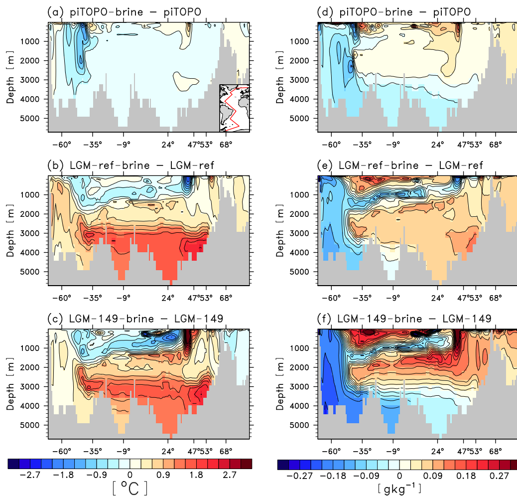
Figure 11. Temperature and salinity changes caused by the reduced brine release. Shown is the same transect through the Atlantic as in Fig. 5. Temperature difference for (a) piTOPO-brine – piTOPO, (b) LGM-ref-brine – LGM-ref and (c) LGM-149-brine – LGM-149. Salinity difference for (d) piTOPO-brine – piTOPO, (e) LGM-ref-brine – LGM-ref and (f) LGM-149-brine – LGM-149. Contour intervals are 0.3°C and 0.03 g kg -1 , respectively.
