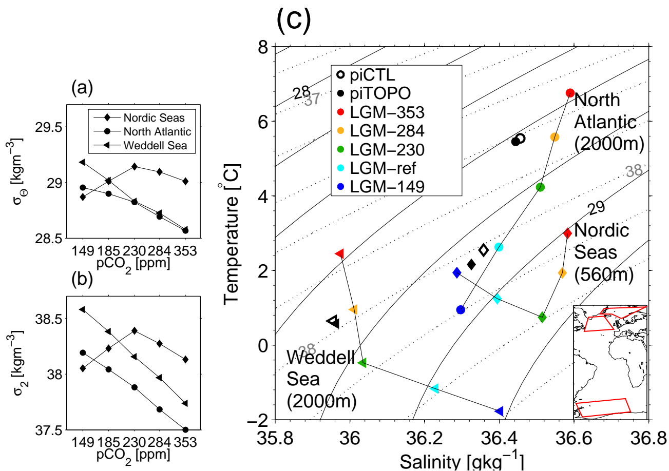
Figure 9. Maximum of (a) \sigma_\theta and (b) \sigma_2 at 560 m in the Nordic Seas and at 2000 m in the North Atlantic and Weddell Sea as a function of p\text{CO}_2 in the glacial setup. (c) Temperature and salinity corresponding to the maximum density in each region. Solid contours indicate \sigma_\theta , dotted contours indicate \sigma_2 . The contour interval is 0.2 \text{ kg m}^{-3} . For an easier comparison with the glacial setup runs, the salinity of piCTL and piTOPO has been offset by 1.21 \text{ g kg}^{-1} to account for the global mean salinity difference caused by the lower glacial sea level. The small map shows the definition of the three selected regions.
