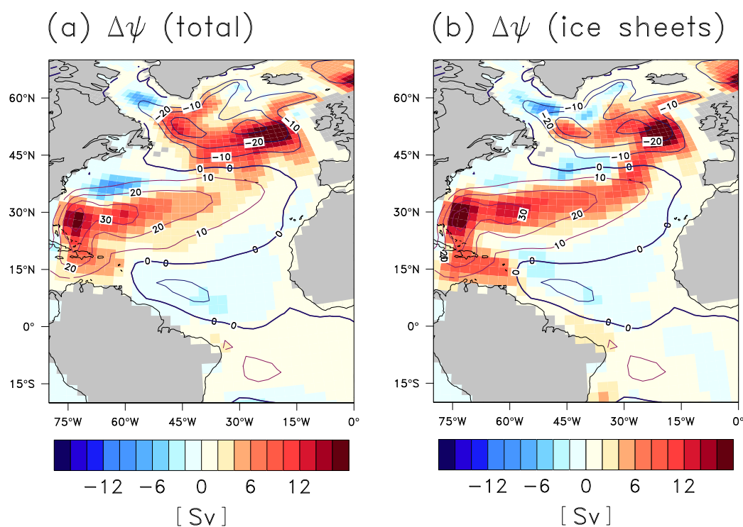
Figure 4. Changes in the barotropic stream function induced by (a) the total glacial forcing (LGM-ref – piCTL) and (b) the ice sheets (LGM-284 – piTOPO). Superimposed contours show the absolute barotropic stream function in the respective reference experiment, i.e., piCTL in (a) and piTOPO in (b). Cyclonic rotation is indicated by blue contours, anti-cyclonic rotation by red contours.
