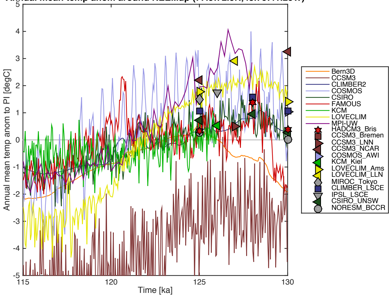
Annual mean temp anom around NEEMup (77.5:72.5N,48.75:41.25W)
