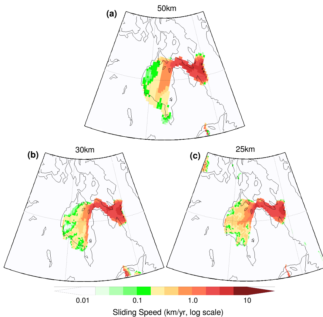
Figure 11. Instantaneous basal sliding speed for model runs at 3 different resolutions, (a) 50km, (b) 30 km, (c) 25km. Colours for speed are plotted on a logarithmic scale.
