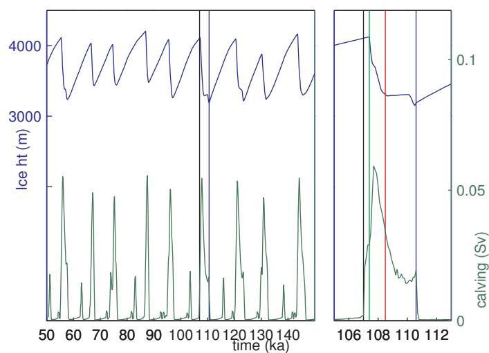
Figure 3. Variability in the ice sheet over Hudson Bay and Hudson Strait. The upper curve shows the average height of the ice sheet over the central Hudson Bay (m, blue box in Fig. 2), the lower curve is the flux of ice out of the mouth of Hudson Strait ( 1 \text{ Sv} = 1 \times 10^6 \text{ m}^3 \text{ s}^{-1} ). The left panel shows results for 100,000 years of model run, the right panel zooms in on the event between 105-113 kyr.
