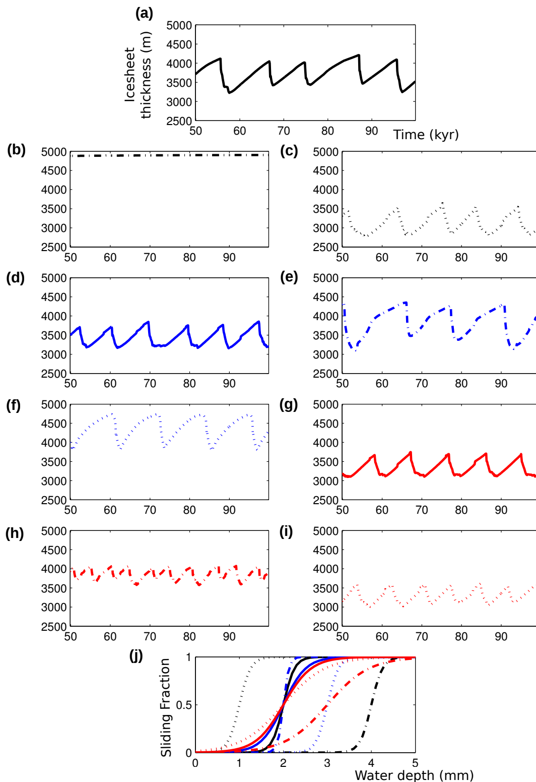
Figure 10. Sensitivity to the parameters (a) and (b) in Eq. 1. These values are presented in Table 2. Panels (a)-(i) show the surface height of the ice sheet averaged over the blue box in Fig 3. Panel (j) shows the sliding fraction, \frac{C}{C_0} from Eq. 1, as a function of water depth, for the different values.
