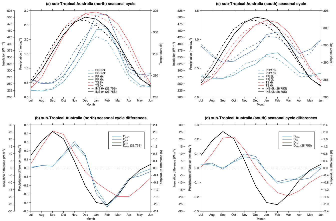
Figure 9. The monthly, ensemble and regional mean insolation (taken at 23.75°S for insolation, black line, W m^{-2} ), surface temperature (red line, K), total precipitation (blue line, mm day^{-1} ) and convective precipitation (turquoise line, mm day^{-1} ) at 0 ka (solid lines) and 6 ka (dashed lines) within (a) the northern half of the sub-tropical arid box and (b) the difference in those same fields for 6 ka minus 0 ka for the northern half of the sub-tropical arid zone. Equivalent figures for the southern half of the sub-tropical arid zone (c and d, insolation at 28.75°S) are also plotted.
