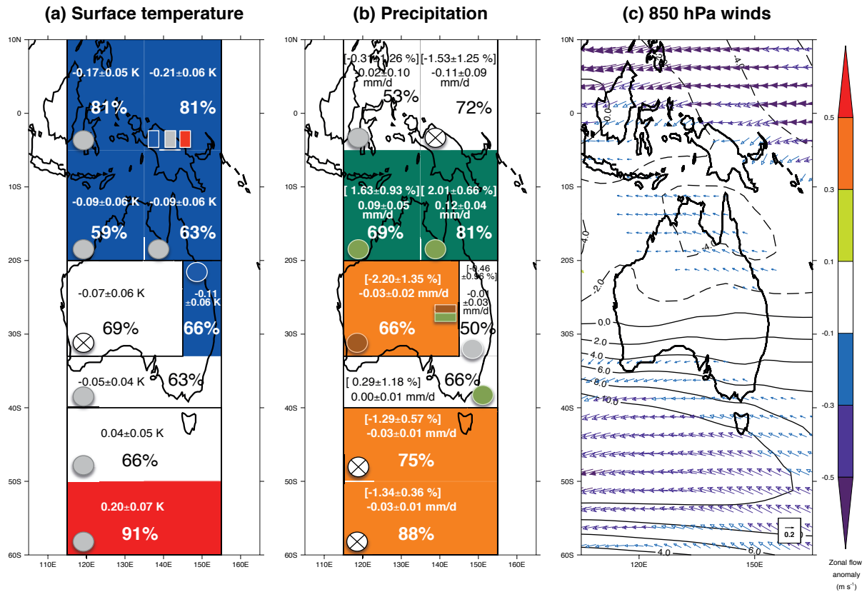
Figure 3. The ensemble and regional annual mean differences in (a) surface temperature (K), (b) precipitation (mm day -1 and [%]) and (c) 850 hPa circulation (m s -1 ) for the 6 ka simulations relative to the 0 ka simulations. In (a) blue shading (circles) indicates lower area-averaged surface temperature and red shading (circles) indicates higher at 6 ka from PMIP (proxy) estimates. In (b), orange shading (circles) indicates lower area averaged precipitation and green shading (circles) indicates higher at 6 ka from PMIP (proxy) estimates. Grey circles indicate that proxy-derived temperature and/or precipitation at 6 ka was equivalent to 0 ka and unshaded boxes indicate changes in temperature and/or precipitation that are not statistically significant ( p > 0.05 ) in the models. N.B. In (a) the blue, grey and red boxes indicate that all three possible states for temperature are possible from the proxy data in the TNE at 6 ka relative to 0 ka; in (b) the orange/green rectangles denote the precipitation change in the northern and southern halves of the StA zone, respectively. In both (a) and (b) the values of the ensemble mean changes [in brackets] and the percentages of models that agree on the sign (positive or negative) of the ensemble mean temperature or precipitation differences are given. Furthermore, circles with an "X" through the middle indicate no proxy data available (both temperature and precipitation). In (c) solid and dashed contour lines indicate mean westerly and easterly flow (respectively) in the 0 ka simulations and the overlaid arrows show vector wind anomalies for 6 ka relative to 0 ka (arrow length and colour is proportional to wind anomaly strength).
