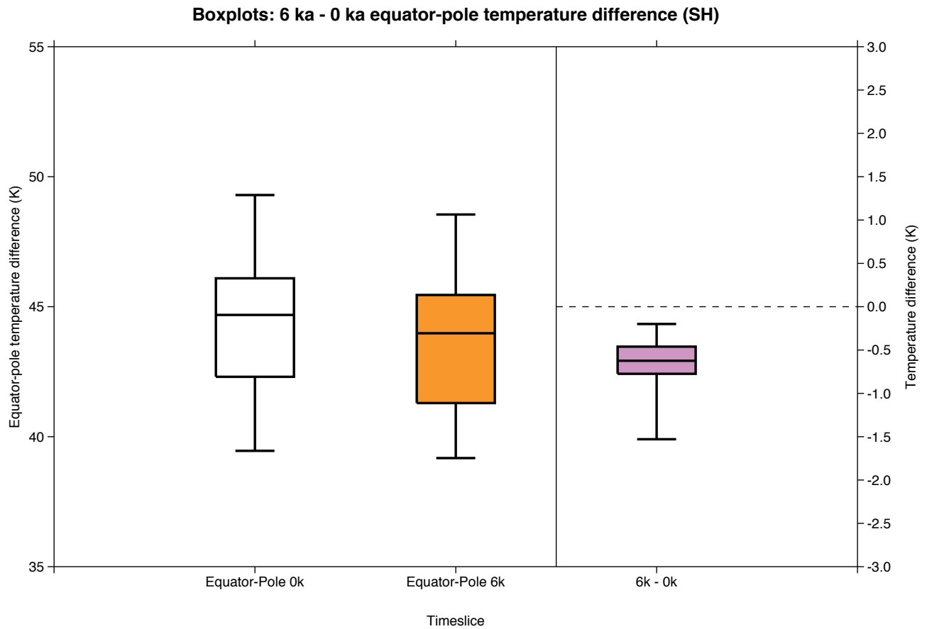
Figure 10. Box-and-whisker plots of the individual model mean difference in surface temperature between 30^{\circ}\text{N} - 30^{\circ}\text{S} and 60^{\circ}\text{S} - 90^{\circ}\text{S} in the 0 ka simulations (white boxes, left axis, K) and the 6 ka simulations (amber boxes, left axis, K). The pink box (associated with the right axis, K) is the individual model difference in the equator to pole temperature gradient for 6 ka relative to 0 ka.
