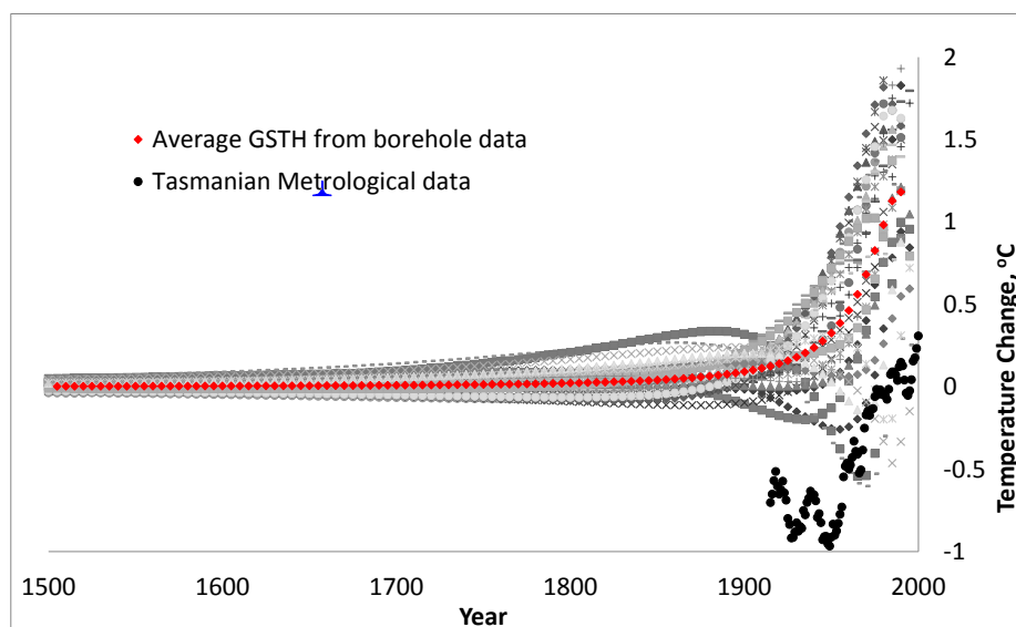
Fig. 7 Reconstructed GSTH from Tasmanian high quality data set, black circles represent average temperatures from meteorological data compiled from surrounding five meteorological stations. Note that the meteorological data has been offset by 1°C for clarity.
