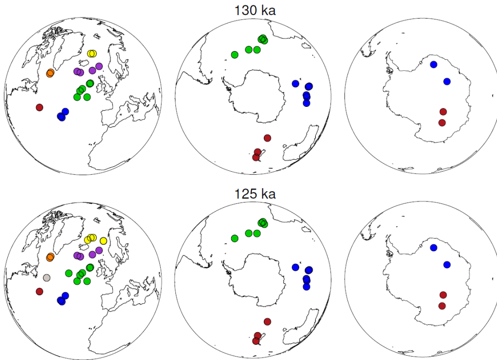
Figure 4. Locations of 130 ka and 125 ka data-based time slice data from Capron et al. (2014). The colors denote the groups of data used in Method 2 (Eq. (2)) to calculate the RMSE for each region.
