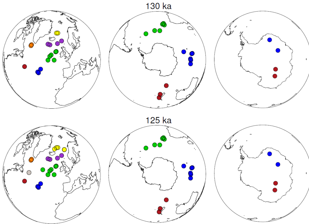
Figure 5. Locations of 130 ka and 125 ka data-based time slice data from Capron et al. (2014). The colors denote the groups of data used in Method 2 (Eq. (2)) to calculate the RMSE for each region.
