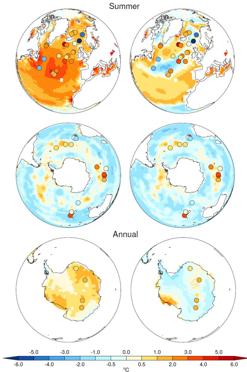
Figure 6. Simulated summer (NH-July, August, September; SH-January, February March) SST and annual (bottom panel) surface air temperature anomalies at 125 ka compared with the Capron et al. (2014) 125 ka data-based time slice. Left panel: HadCM3, right panel: NorESM. Table 2 shows a similar agreement with data for NorESM and HadCM3 (which has no cooling in the North Atlantic) in the NH when compared with the 125 ka data-based time slice from Capron et al. [2014]. However, NorESM shows poor agreement with the data synthesis over Antarctica. Anomalies calculated relative to the preindustrial for the model and relative to xxx for the data.
