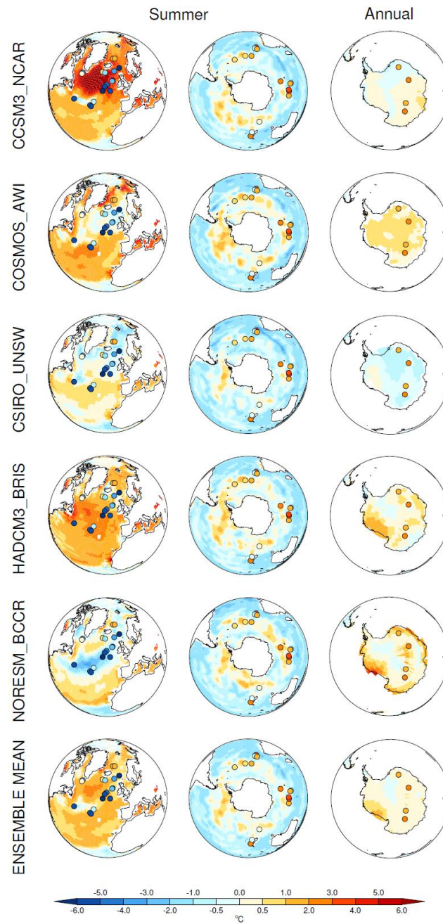
Figure 2. Simulated summer (NH-July, August, September; SH-January, February March) (left and middle panels) SST and annual (right panel) surface air temperature change relative to preindustrial, for GCM model results previously published (Lunt et al., 2013) and their ensemble mean. The simulations are compared with the new data-based 130 ka time slice (Capron et al., 2014).
