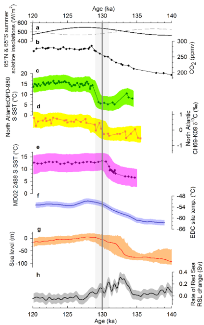
Figure 1. (a) 65°N (black) and 65°S (grey) summer insolation (Laskar et al., 2004). (b) EDC ice core CO 2 concentration (Schneider et al., 2013) (black). (c) North Atlantic core ODP-980 summer-SST reconstruction (Oppo et al., 2006) (green) and associated 2σ uncertainty envelope (Capron et al., 2014) (light green). (d) North Atlantic core CH69-K09 δ 13 C record (Govin et al., 2012 and 2σ uncertainty envelope (this study, see details on the methodology in Capron et al., 2014)). (e) Southern Ocean core MD02-2488 summer-SST reconstruction (Govin et al., 2012) (pink) and 2σ uncertainty envelope (Capron et al., 2014) (light pink). (f) EDC surface temperature reconstruction (dark blue) and associated 1.5°C uncertainty envelope (Masson-Delmotte et al., 2011) (light blue). Ice and marine sediment records (a-d) are presented on the AICC2012 ice core chronology (Bazin et al., 2013; Capron et al., 2014; Veres et al., 2013). (f) Note that Govin et al. (2015) reports in the Table 5 of their paper that the Antarctic reconstructed surface temperature (based on EDC dD) starts increasing at 135.6 ± 2.5 ka based on the use of the RAMPFIT software. (g) Red Sea relative sea level (RSL) data (probability maximum, red) with 95% confidence interval (Grant et al., 2012) (orange). (gh) Red Sea rate of RSL change (probability maximum for the first-order time derivative, in meters/kyr/Sv, black) with 95% confidence interval (Grant et al., 2012) (grey). Note that ice and marine records from (a) to (ef) are shown on the AICC2012 ice core chronology (Bazin et al., 2013; Capron et al., 2014; Veres et al., 2013) while the Red Sea records (f-g, h) are displayed on their original age scale which is independent from the AICC2012 ice core chronology (see Grant et al., 2012 for details) The grey vertical line marks 130 ka. The grey band highlights the 129-
