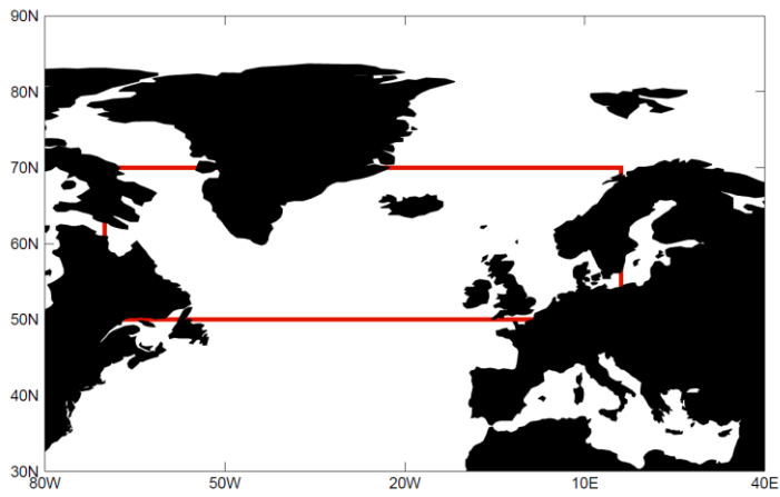
Figure 3. The North Atlantic region for freshwater input denoted by the red box (50-70°N). Note that the freshwater amount is evenly distributed within this region.
