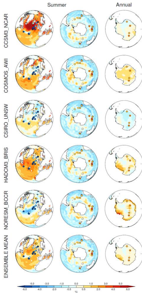
Figure 2. Simulated summer (NH-July, August, September; SH-January, February March) (left and middle panels) SST and annual (right panel) surface air temperature change relative to present-day preindustrial , for GCM model results previously
