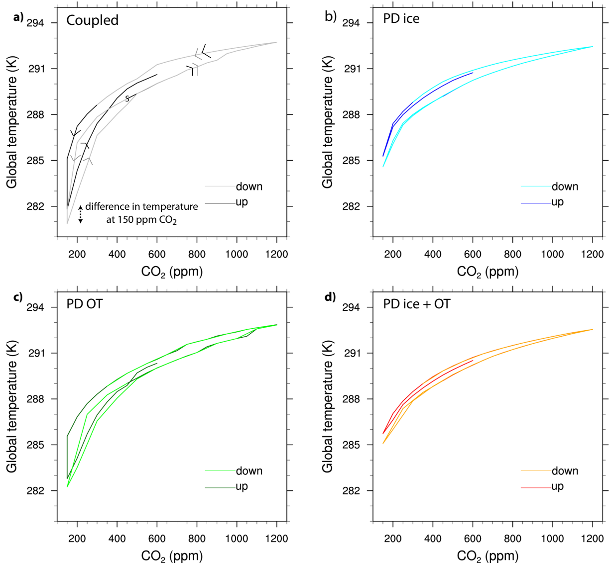
Figure 3. Relation between CO 2 and global temperature in the equilibrium runs. In (a), the fully coupled model output is shown. The starting point of the simulation at 450 ppm CO 2 is marked by an S, and the consequent evolution for both runs is marked by coloured arrows. The black line shows the up run, where CO 2 is increased first, the grey line shows the down run, where CO 2 is decreased first. At high CO 2 levels, the black line is overlaid by the grey line. In (b) the output with uncoupled ice (blue/cyan), in (c) with uncoupled ocean overturning strength (darkgreen/green) and in (d) with both these factors uncoupled (red/orange) are shown. The darker colors (blue, darkgreen, red) show the up runs, the lighter colors (cyan, green, orange) show the down runs. The startpoint and evolution are the same as in (a).
