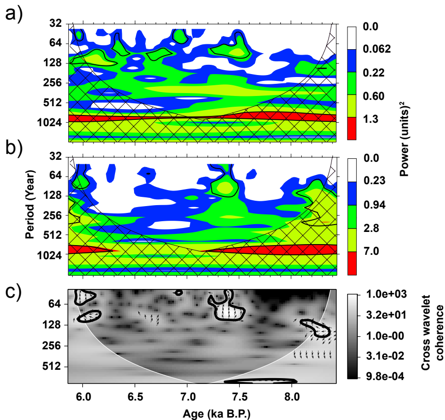
Figure 10. Continuous wavelet transform of (a) assemblage-based summer SST and (b) Mg/Ca-based upwelling SST. The 10% significance level against red noise is shown as black contour lines. (c) Cross wavelet transform (XWT) of the trend-removed Mg/Ca-based and assemblage-based SST time series. The 5% significance level is shown as thick contours. Relative phasing of both records is indicated by arrows. Arrows within the significant intervals pointing mostly upwards, which indicates a consistent phase-shift of both records by 90° or 270°, respectively, of assemblage-based SST relative to Mg/Ca-based SST. The cone of influence, where edge artefacts might be introduced, is indicated by hatching and white shading, respectively.
