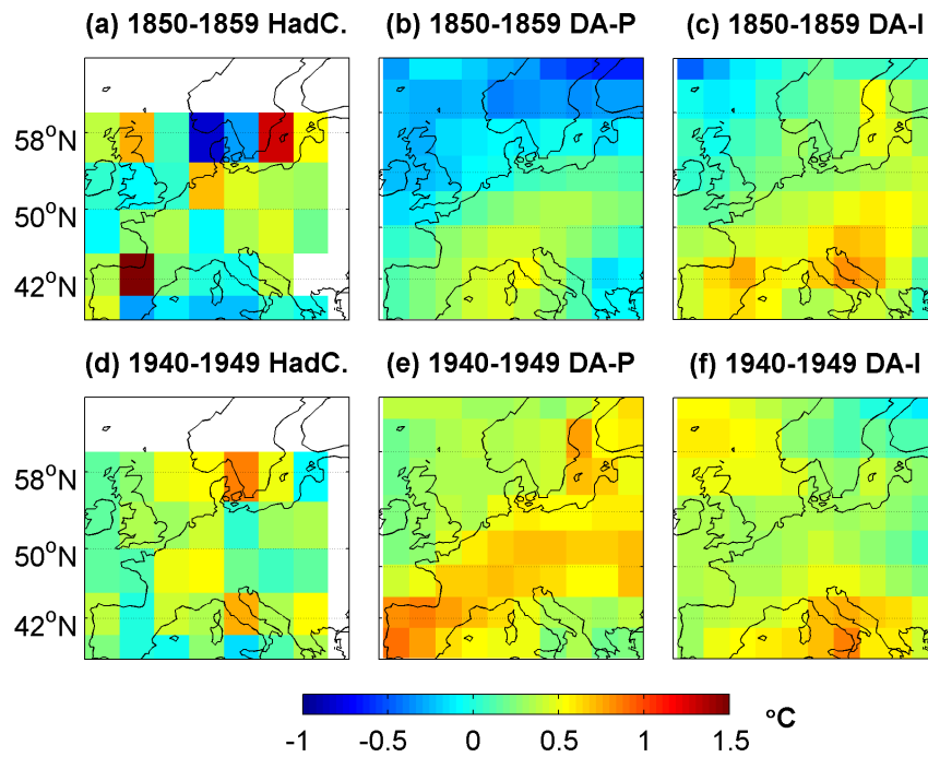
Figure 4. European decadal surface air temperatures (anomalies w.r.t. the 1850-1949 AD mean) for the DA-P analysis, the DA-I analysis and the HadCRUT3v reconstructions, for the summers of 1850-1859 AD and 1940-1949 AD.
